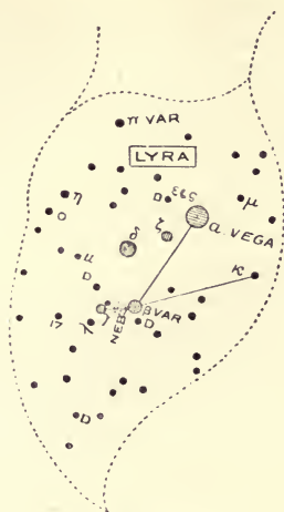
Fig. 1.—The Constellation Lyra.
