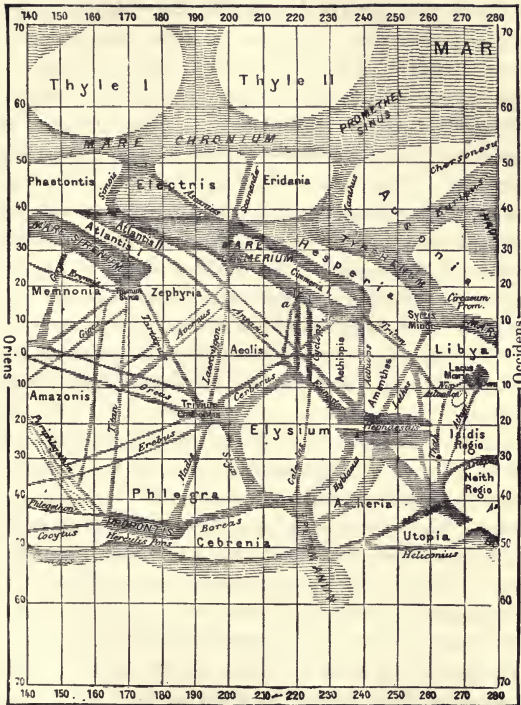
Fig. 21.—Part of a Map of Mars.
