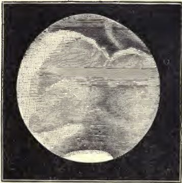
Fig. 20.—Mars through the telescope.
