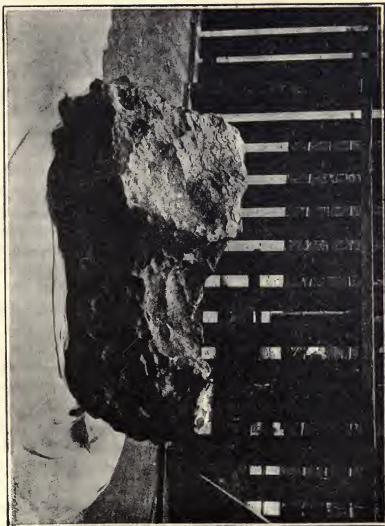
Fig. 35.—The large Youndegin Meteorite. 4 feet 2 inches long, 2 feet 3 inches wide, 20 inches thick. Weight 2,044 lbs. (18½ cwt.).
