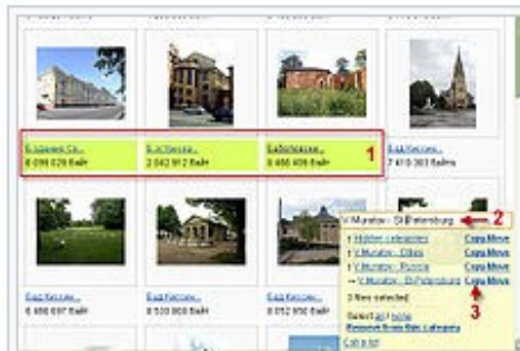
Figure 1: Cat-a-lot steps:
