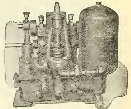
Fig. 1705—Power Sprayer with Automatic Governor.
