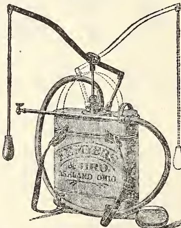
Fig. 547.—No. 330 Galvanized.
