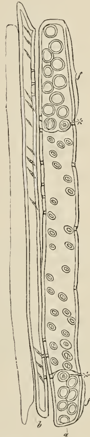
FIG. 59.— Ephedra helvetica . Wood (23a); a member of a vessel, b tracheides seen from the radial side, isolated by maceration with Schultze's mixture; f the oblique ends of the member of the vessel in surface view, with two rows of large open bordered pits; at x, x two closed bordered pits. Of the tracheides, b is only drawn in outline, the surface of the other is put in. (The direction of the split-like pits is reversed; they rise in reality from left to right.)
