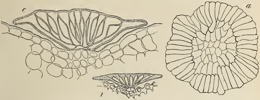
FIG. 41.— a, b Rhododendron ferrugineum ; glandular scales of the under surface of the leaf. a surface view of a larger one; b transverse section of a smaller one (142). In the latter the cells are shaded; the intervening spaces filled with secretion, not shaded.— c Rhododendron hirsutum ; glandular scales from the under surface of the leaf, transverse section (225). The cellulose membrane of the scale dotted, cell-contents and secretory space left white; over the cellulose membrane runs the cuticle, which is connected with that of the surrounding epidermis. In all cases the secretion has been removed by alcohol.
