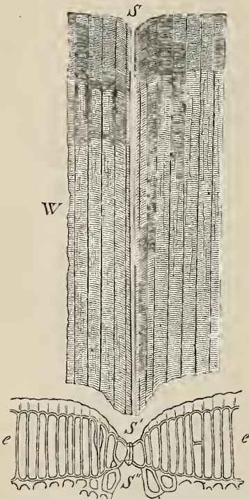
FIG. 30.—(116) Klopstockia cerifera ; intermode of stem, transverse section. e —epidermis; S-S' stoma, with two small guard-cells between the two larger subsidiary cells; w wax covering over the epidermis, over which it fits; S-S' the canal leading to a stoma.
