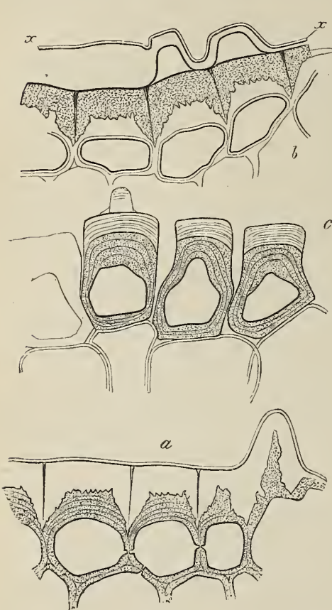
FIG. 25.—(390) Transverse section through the leaf of Aloe verrucosa . a lying in water, not acted upon by reagents. The non-cuticularised parts of the membranes shaded; outside this the cuticular layers, broken up by darker limiting lamellæ, and covered by the cuticle, which has a double contour. b after warming with potash solution. The cuticle x-x raised from the (shaded) cuticular layers; the non-cuticularised (unshaded) inner layers somewhat swollen. c epidermal cells after complete removal of the cuticle, and of the cutin deposited in the cuticular layers, by continued boiling with potash. They are separated from one another, and are seated upon the cells of the sub-epidermal parenchyma; the cuticular layers are now only distinguishable from the others by more delicate stratification.
