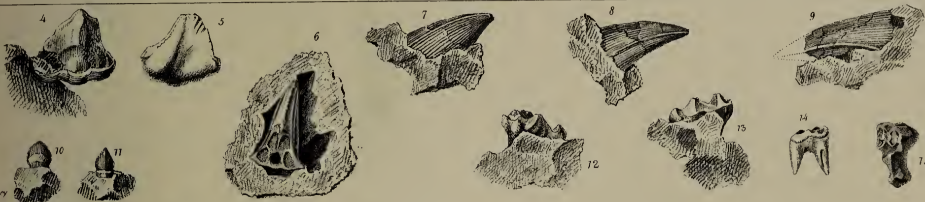
Fossil Teeth found by Lieut ant Cautley in the Lower Range on the S.W. or plainward base of the Himalayas.
