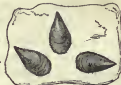
Lingula acuminata
