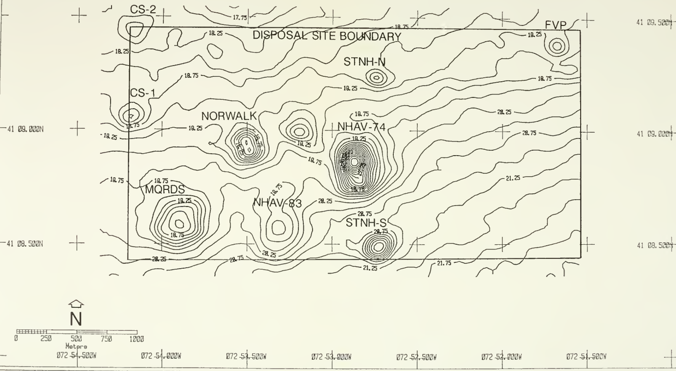
Figure 3-1 Contour bathymetric chart of CLIS Disposal Site, August 1985.
