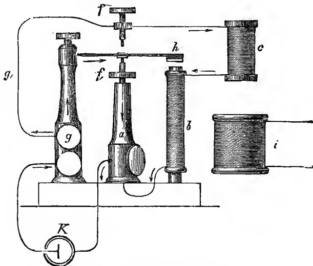
FIG. 74. HELMHOLTZ'S APPARATUS.
