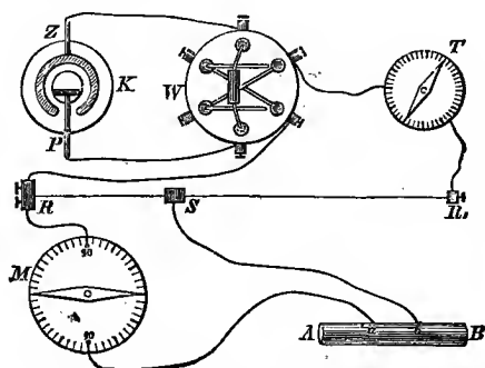
FIG. 46. MEASUREMENT BY COMPENSATION OF THE DIFFERENCE OF TENSION.
