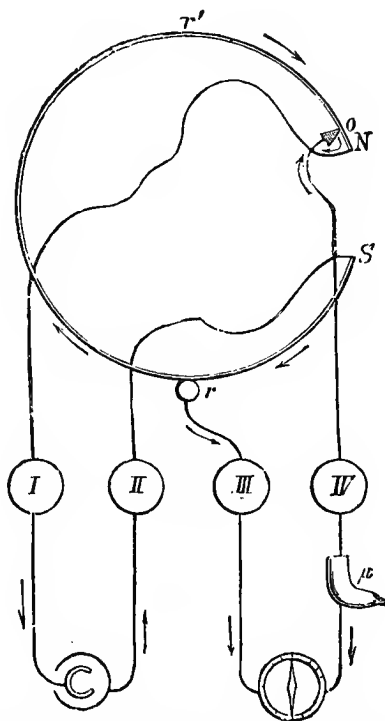
FIG. 48. DIAGRAM OF ELECTRIC MEASUREMENT BY MEANS OF A ROUND COMPENSATOR.
