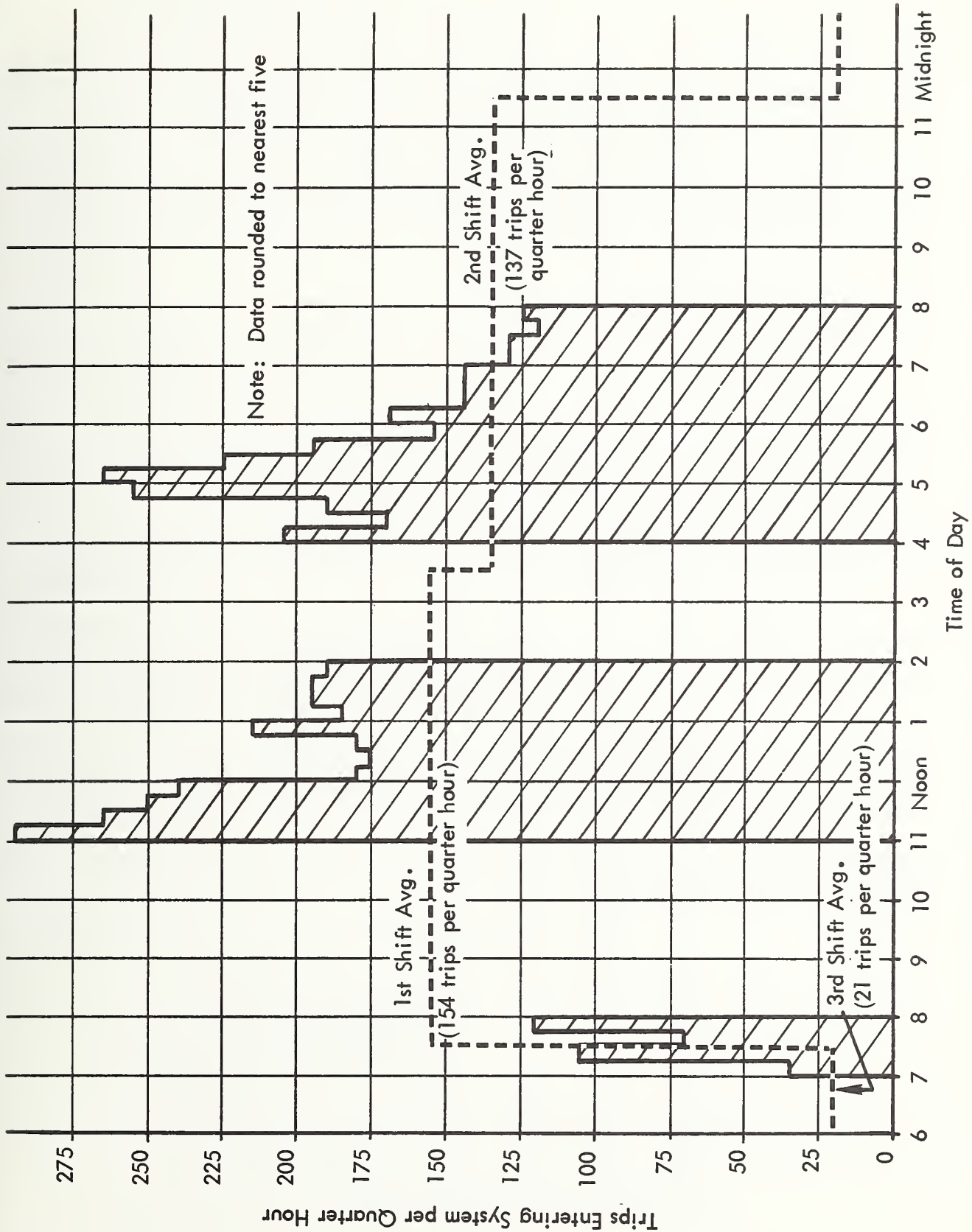
FIGURE 3-3. AIRTRANS DEMAND PROFILE (1974 Passenger Flow Study Data)
