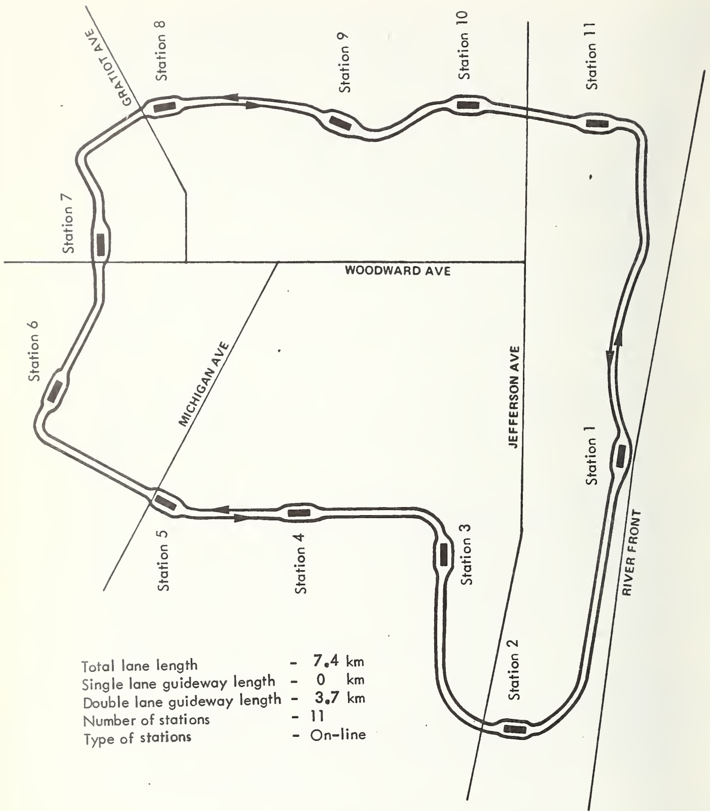
FIGURE 4-4. SLT 4: MEDIUM-DEMAND CBD CIRCULATION APPLICATION USING A LOW-SPEED IGRT ON A TWO-WAY LOOP
