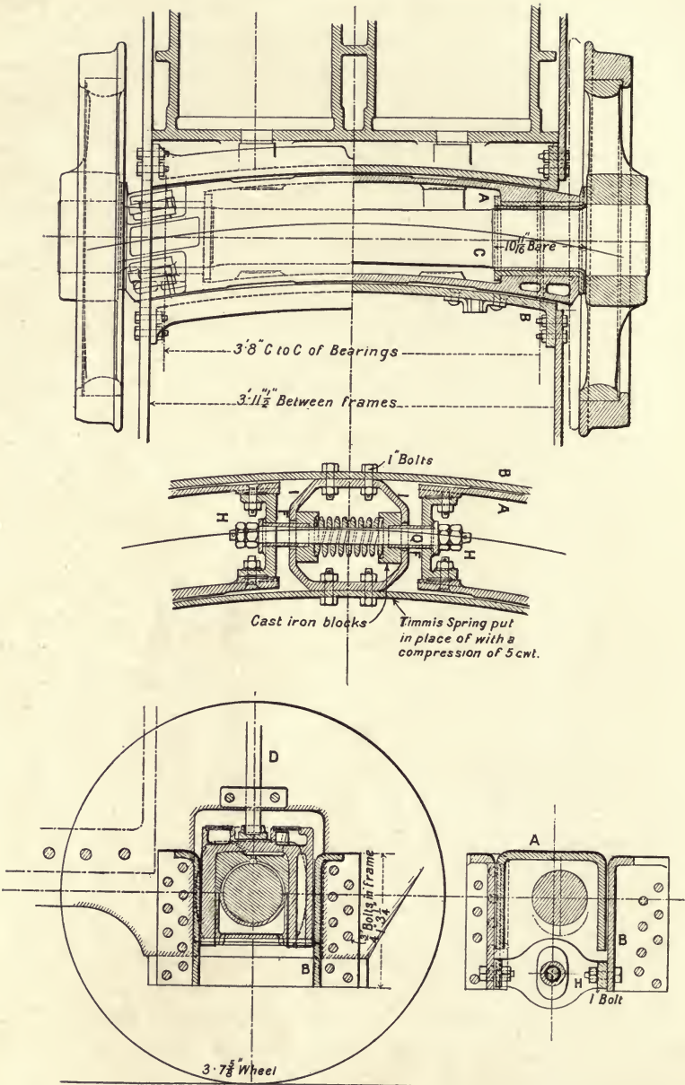
FIG. 29.—Traversing leading axle, Lancashire and Yorkshire Railway.
