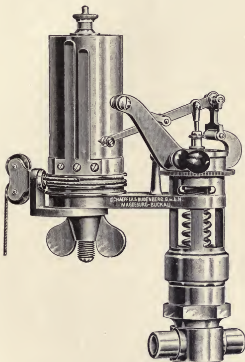
FIG. 82.—Thompson indicator with open spring.
