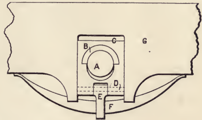
FIG. 17.—Axle-box.
