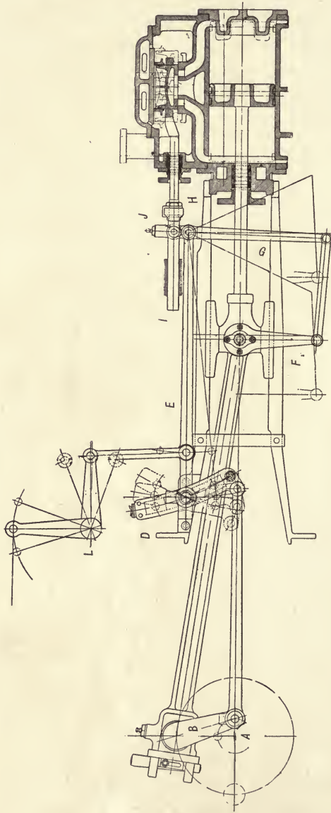
Fig. 79.—Walschaert's gear.
