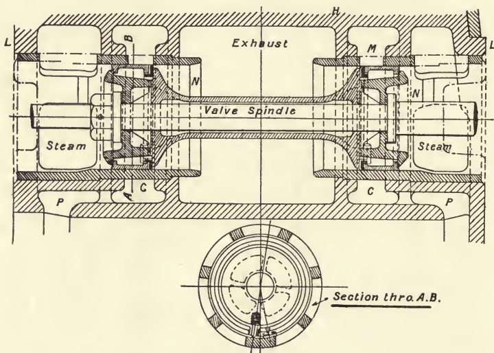
FIG. 81.—Smith's piston valve.
