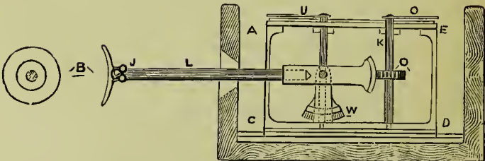
FIG. 4.—Sectional side elevation.
