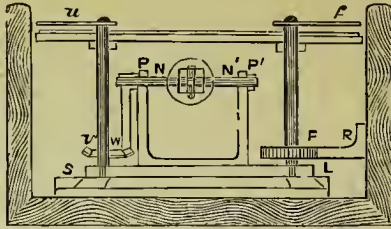
FIG. 2.—Sectional plan and elevation of the three-plane instrument.
