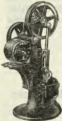
Fig. 47E.—DEEP WELL PUMPING HEAD.
