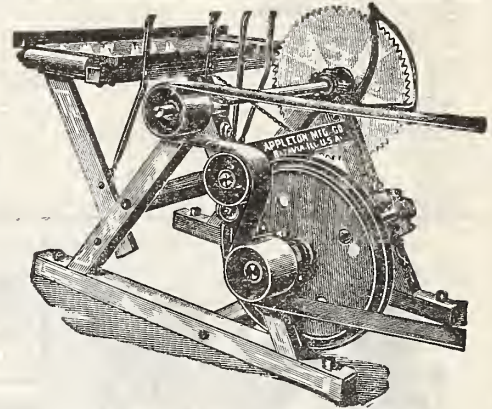
New Style Tilting Table Pole Saw.
