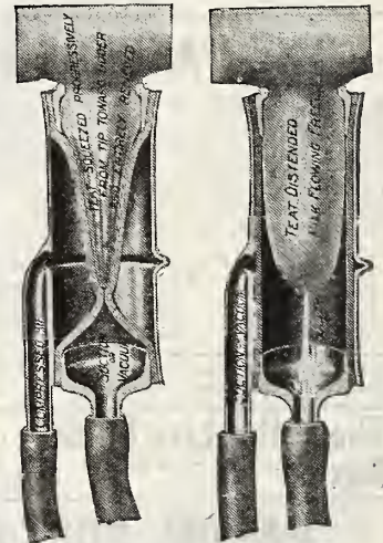
Teat Cups Showing Upward Squeeze.
