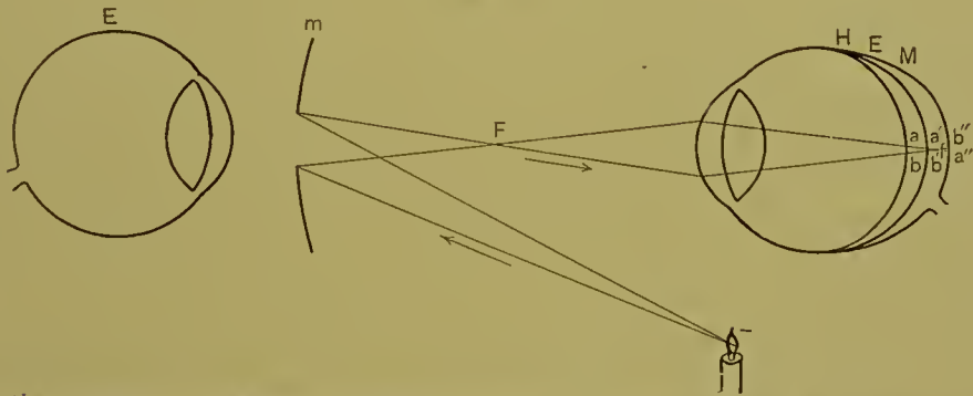
Relative areas and positions of retinal illumination whilst employing the concave mirror.
