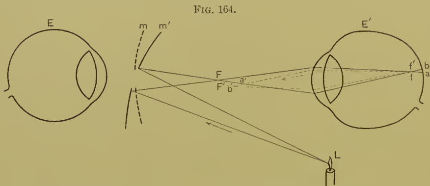
Direction of movement of reflex whilst employing the concave mirror in myopia.
