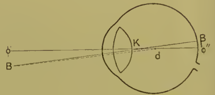
Visual line. Angles alpha and gamma.
