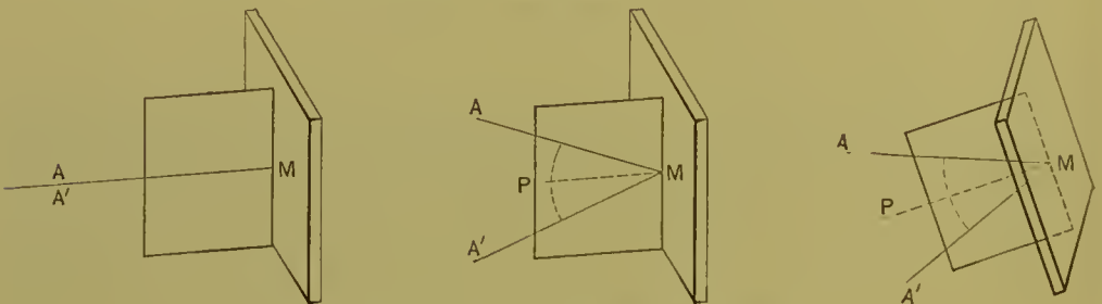
Variations in lines of incidence and reflection.
