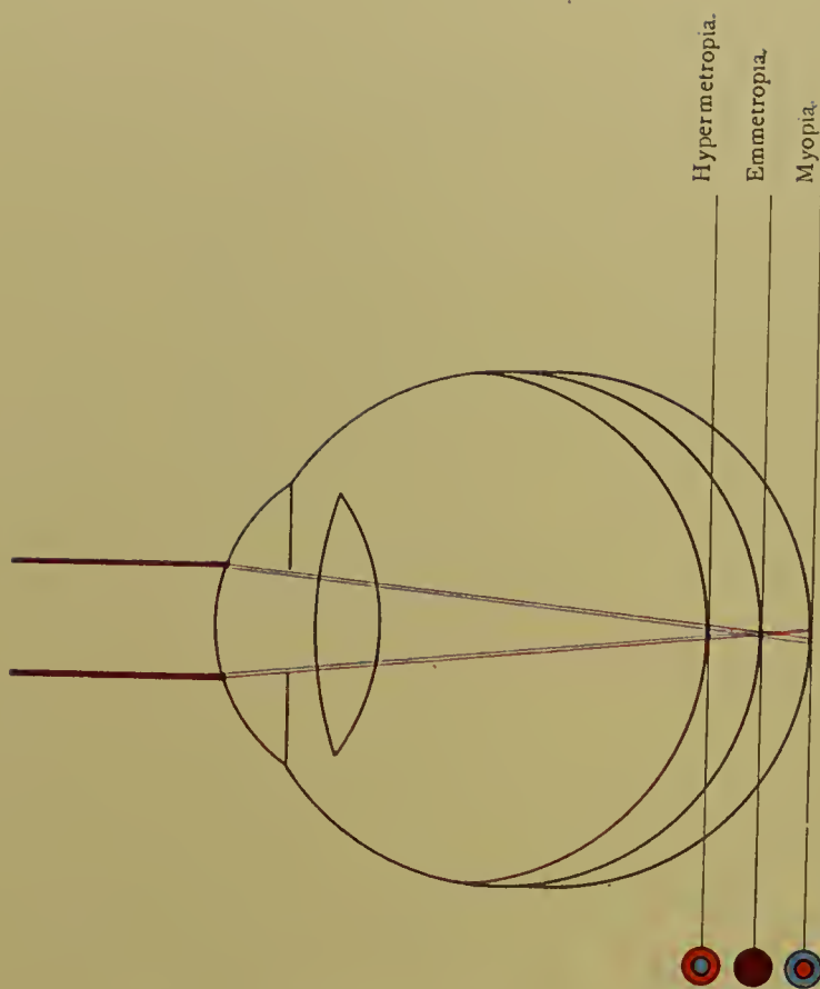
Diagram illustrating chromatic-aberration test for ametropia.
