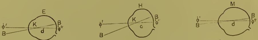
Relative sizes of angle alpha. (Modified from DONDEERS.)
