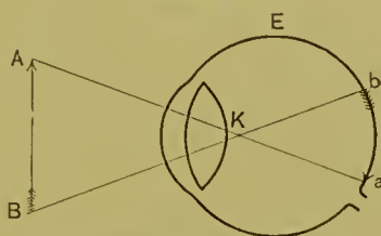
Increased visual angle.
