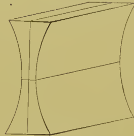
Bi-concave cylindrical lens.
