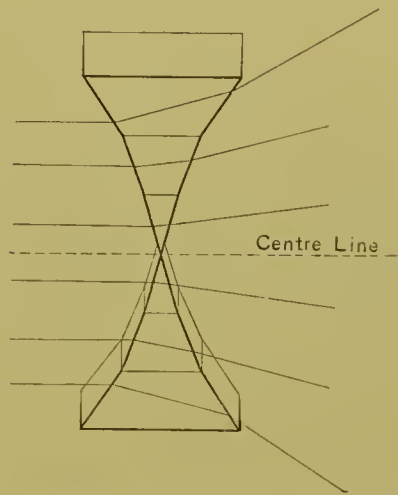
Passage of six parallel rays through six truncated prisms with their bases pointing outward, causing a divergence.
