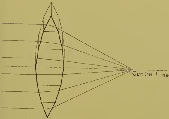
Passage of six parallel rays through six truncated prisms with their apices pointing outward, forming a compound focus.
