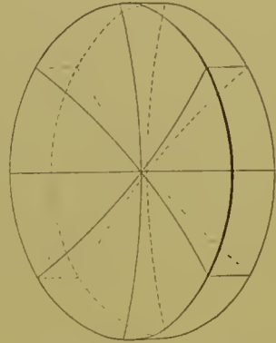
Bi-concave spherical lens.
