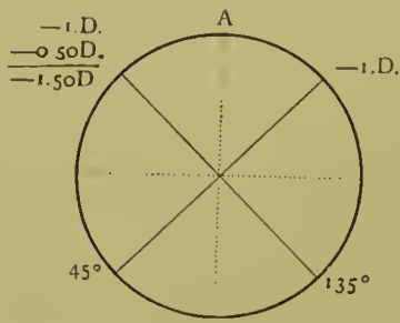
Scheme for graphic determination of lens-powers.
