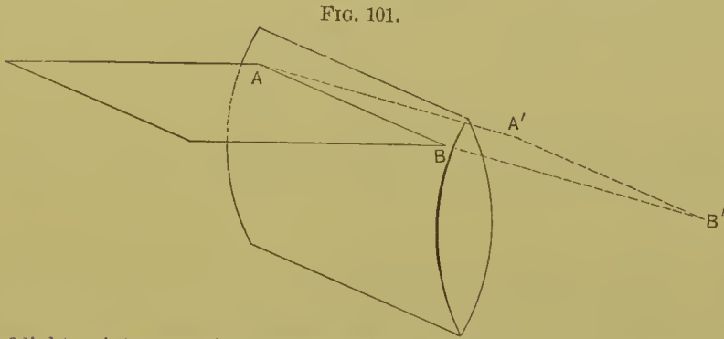
Plane of light uninterruptedly refracted through an excentric portion of the axis of a bi-convex cylindrical lens.
