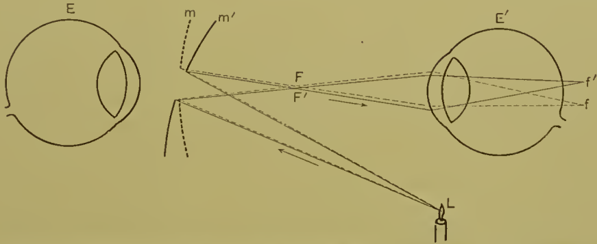
Direction of movement of reflex whilst employing the concave mirror in emmetropia.
