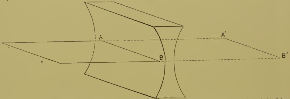
Plane of light passing undeviatingly through the mid-axis of a bi-concave cylindrical lens.
