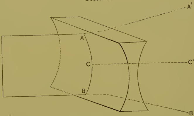
Plane of light passing through a bi-concave cylindrical lens in a meridian at right angles to the lens, dispersed into more widely separate rays.
