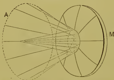
Real focus of highly convergent rays from a convex mirror.
