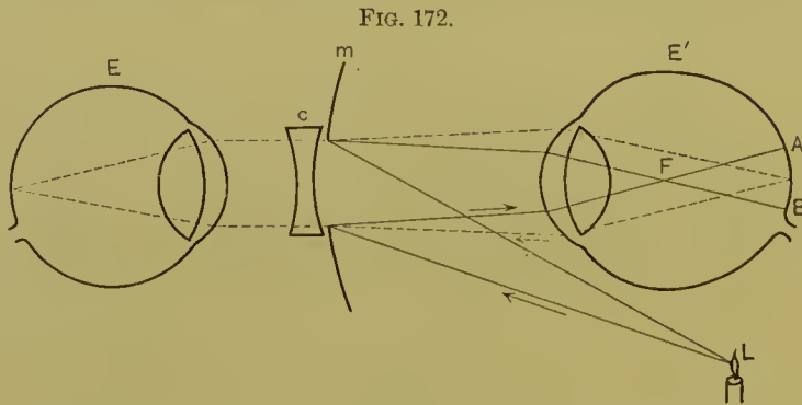
Direction of rays of light by the direct method in corrected myopia.
