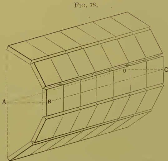
Evolution of a concave and convex cylindrical surface.
