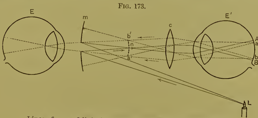
Lines of rays of light by the indirect method in emmetropia.
