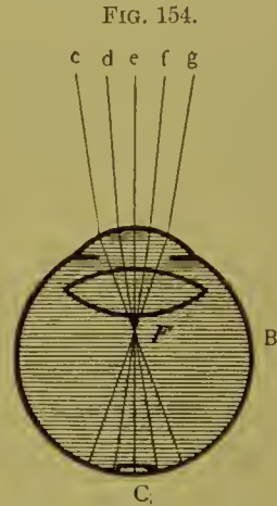
Greatly lessened area of visibility of coin in bottom of a more greatly curved topped medium of increased density—practically an eye.
