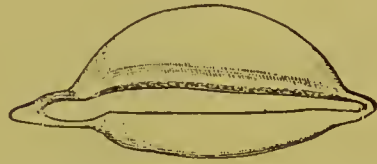
Shape and size of tarsus. (SCHWALBE.)
