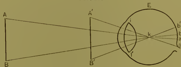
Comparative sizes of retinal images.
