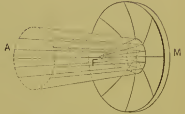
Real focus of convergent rays from a concave mirror.
