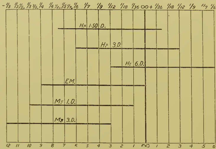
Range of accommodation in emmetropia, hypermetropia, and myopia. (Modified from DONDEBS.)
