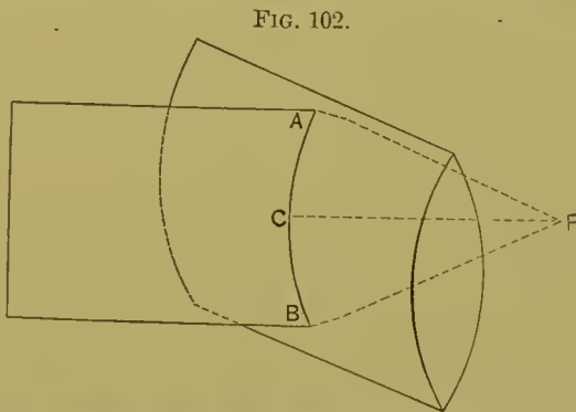
Plane of light passing through a bi-convex cylindrical lens in a meridian at right angles to the axis of the lens, refracted to a point.
