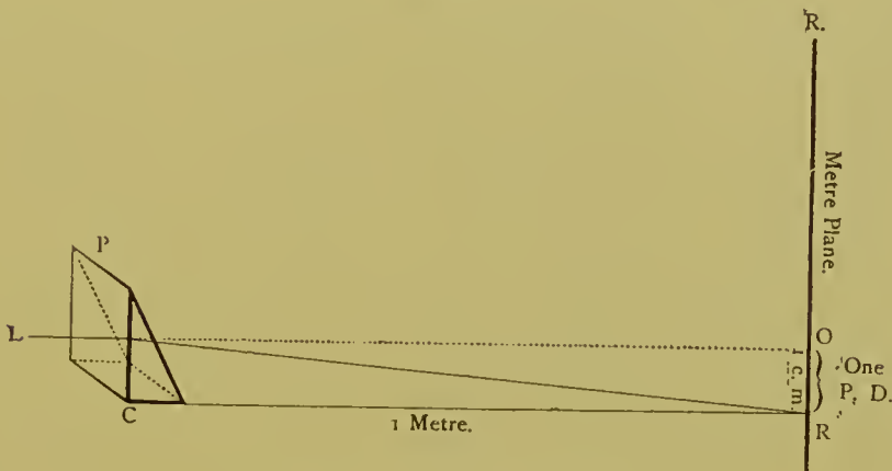
Prism diopter and meter plane.
