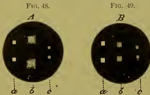
Catoptric images. (HELMHOLTZ.)
