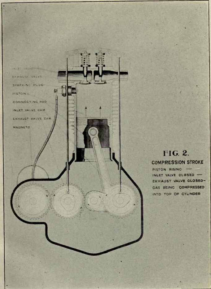
FIG. 2. — Diagram illustrating the Compression Stroke.
