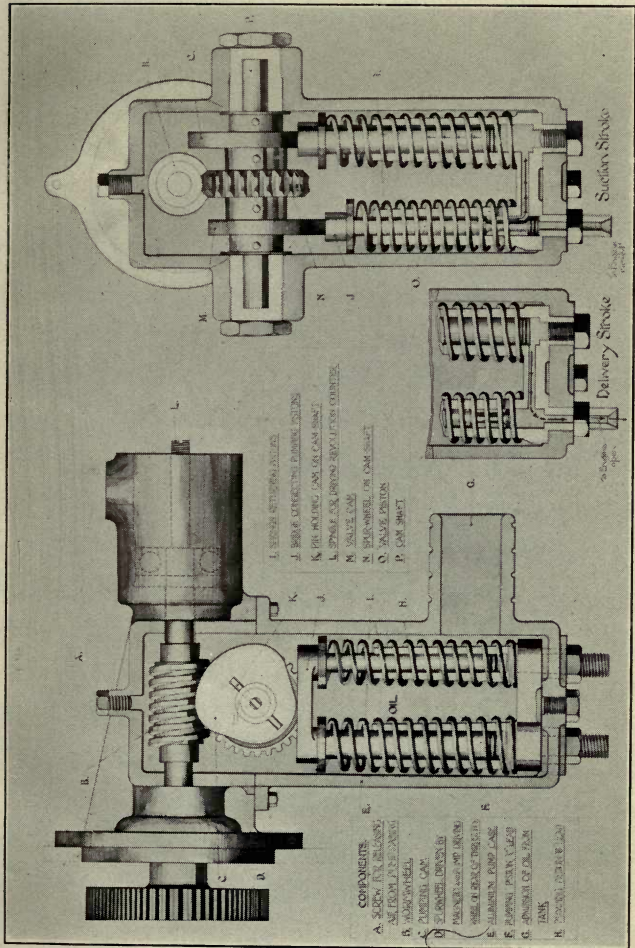
FIG. 8. — Plunger Type Pump.
