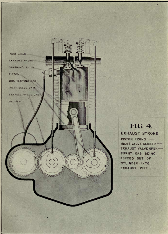
FIG. 4. — Diagram illustrating the Exhaust Stroke.
