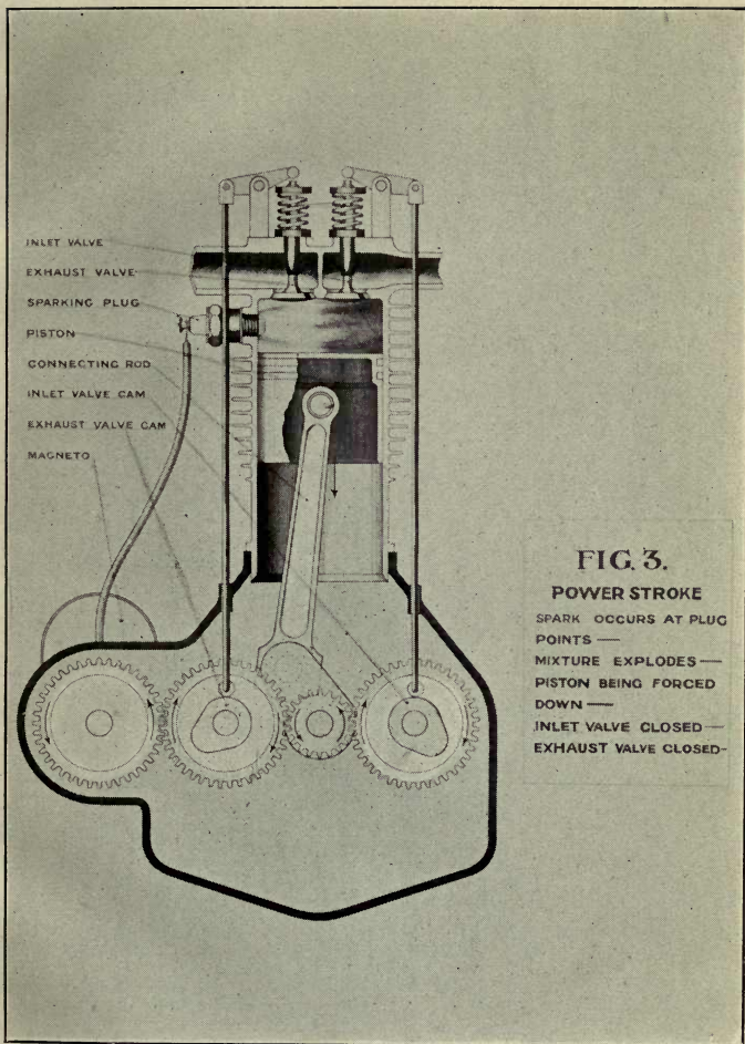
FIG. 3. — Diagram illustrating the Power Stroke.
