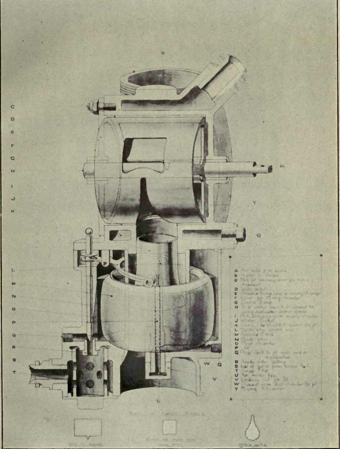
FIG. 17. — The Beardmore Carburetor.
