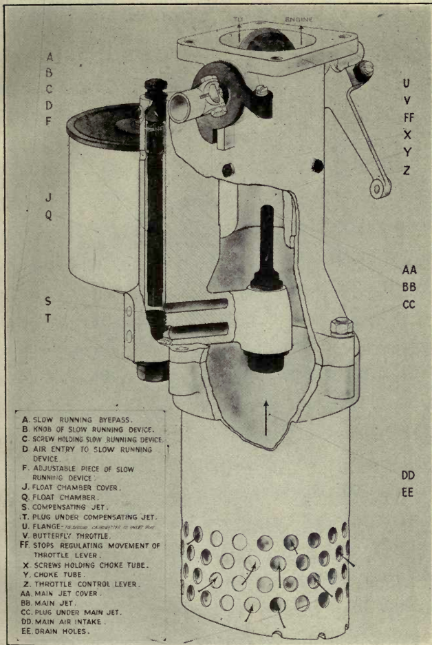
FIG. 18. — Zenith Carburetor.
