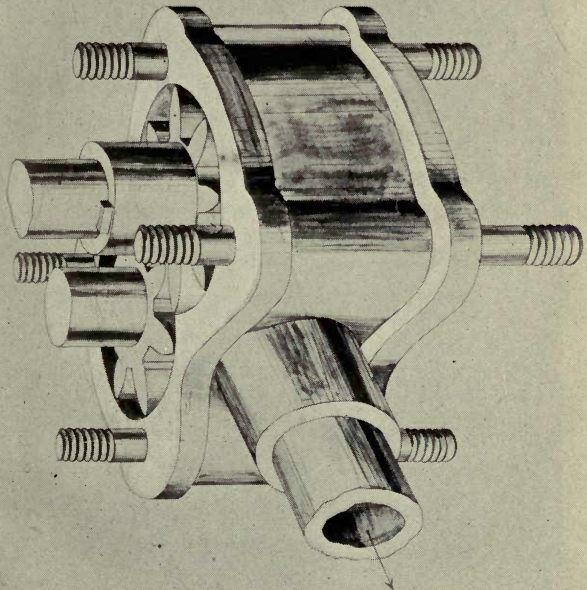
FIG. 7. — Rotary or Gear Type Pump.
