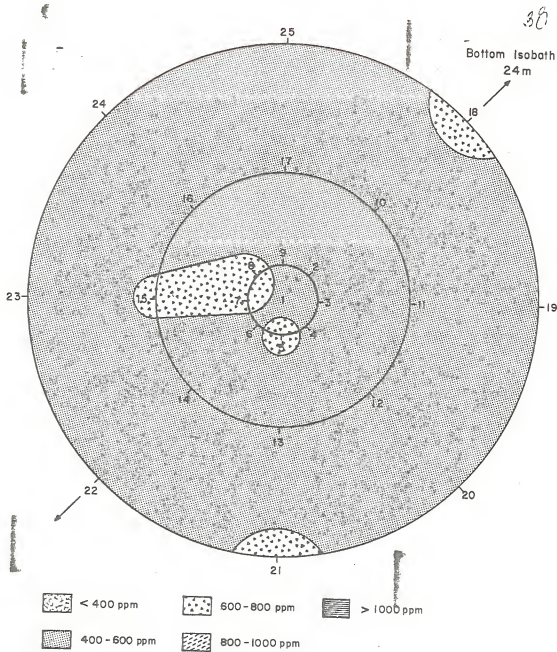
Figure 11a. Distribution of barium (pre-drilling).
