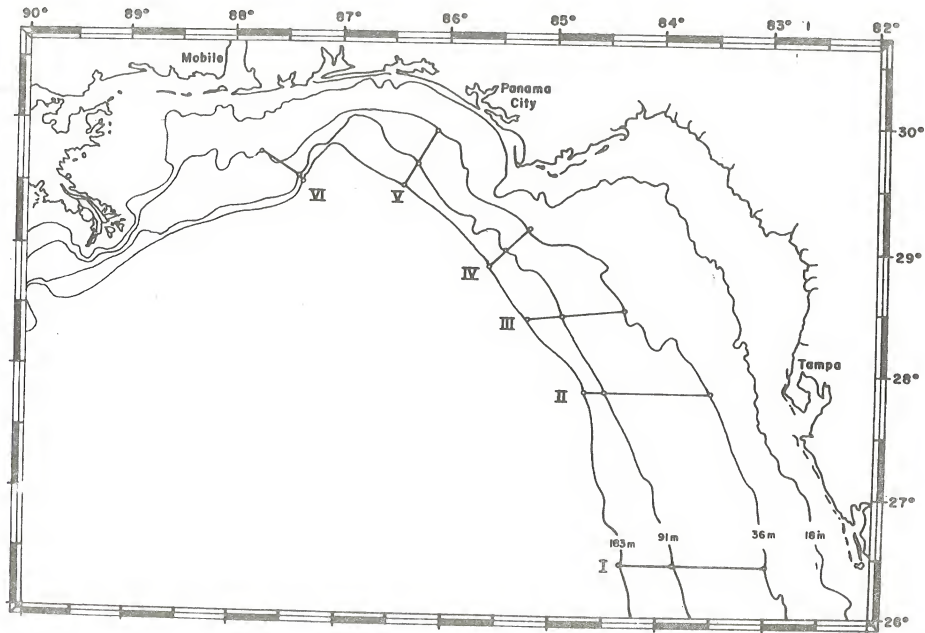
Figure 5. MAFLA dredge/trawl stations, 1975-1976.
