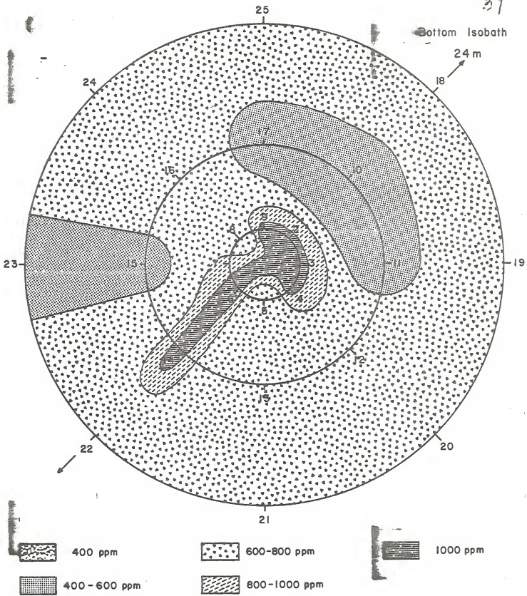
Figure 11b. Distribution of barium (during drilling).
