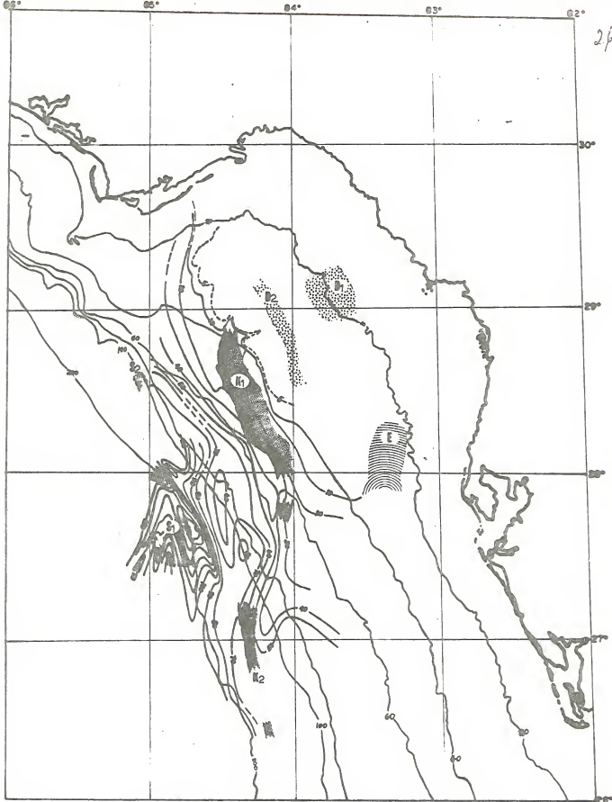
Figure 9. Various subsurface structures located on the peninsula. a Florida shelf. D 1 and D 2 : areas of doline karst features; K 1 and K 2 : karren karst trends; S 1 and S 2 : slope instability evidenced by creep or slumping; E: major filled valley complex; "raw time": thickness of past Miocene strata given in 10 msec contour intervals.
