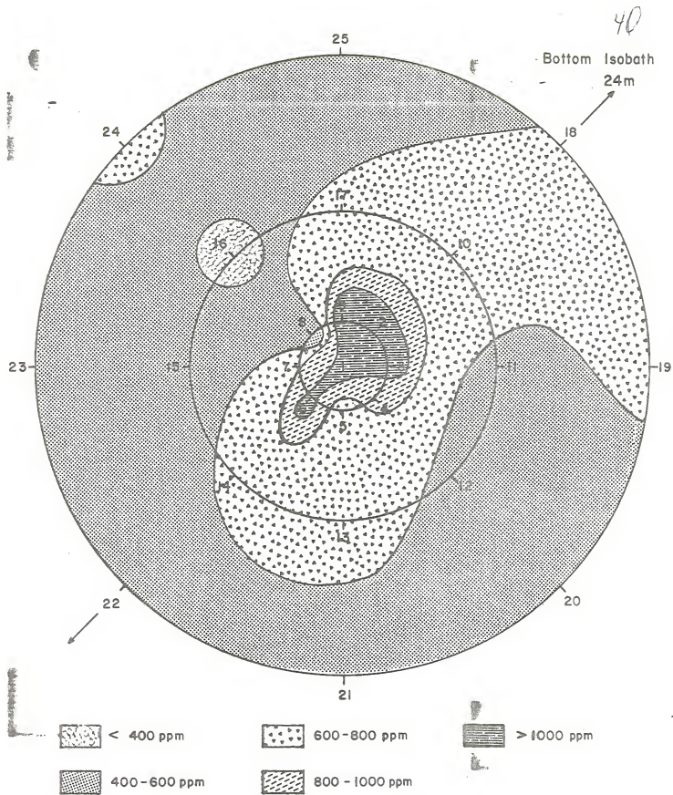
Figure 11c. Distribution of barium (post-drilling).
