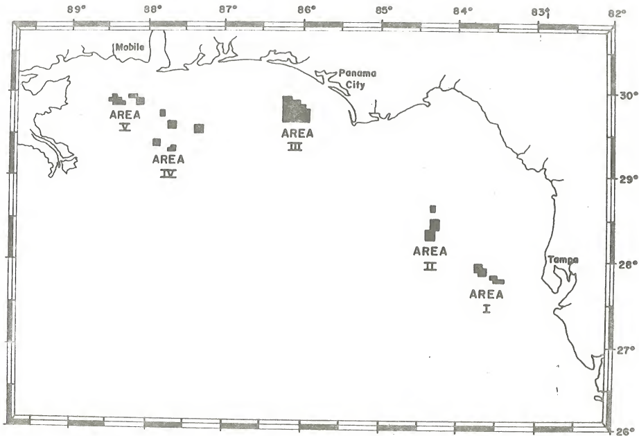
Figure 1. MAPIA benchmark study area.
