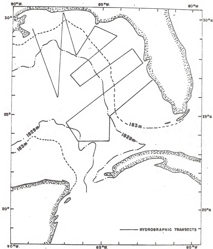
Figure 2. Recommended hydrological transects.
