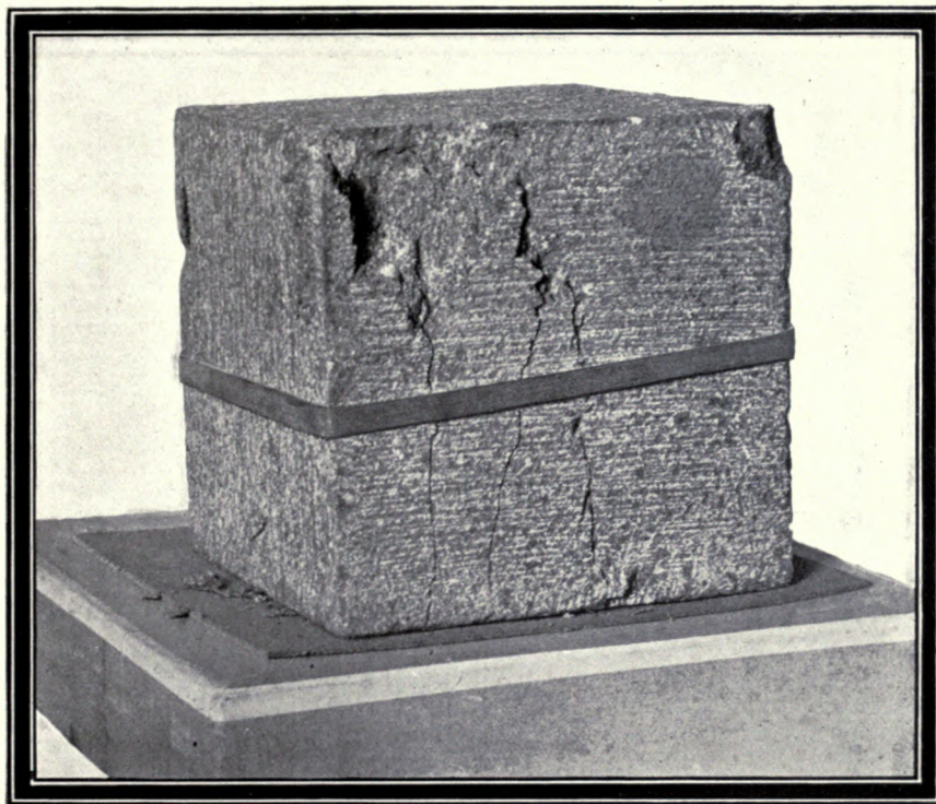
BOWRAL TRACHYTE N.S.W. 3 IN. CUBE CRUSHED AT 84.33 TONS (J. NANGLE).
