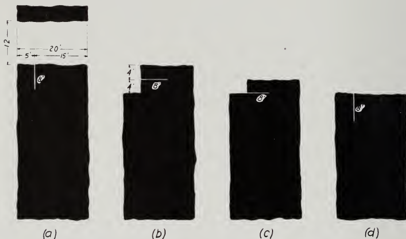
FIG. 18. Method of drawing pillars in District III
