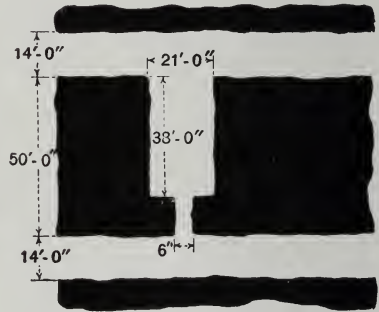
FIG. 14. Crosscut in District VII to provide small stopping
