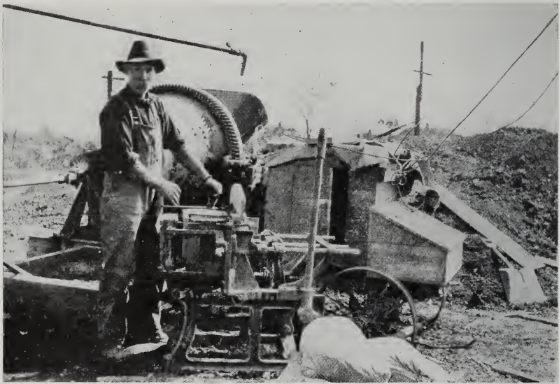
FIG. 51. Mixer and mould for making concrete blocks
