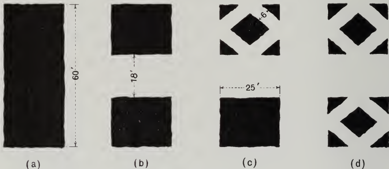
FIG. 19. Method of drawing pillars in District VI
