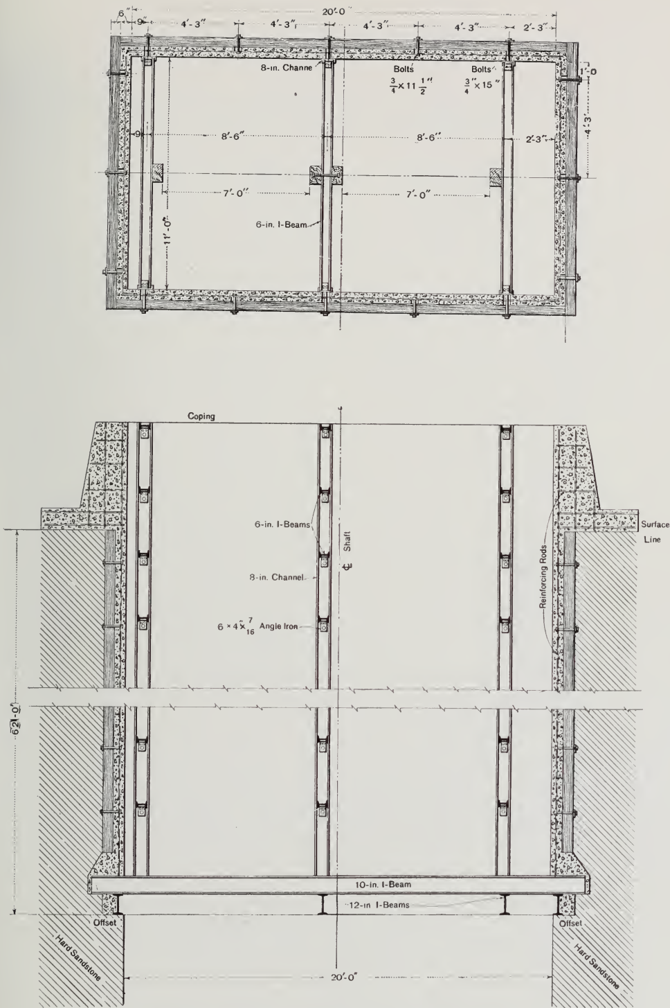
FIG. 62. Plan and section of concrete-lined shaft
