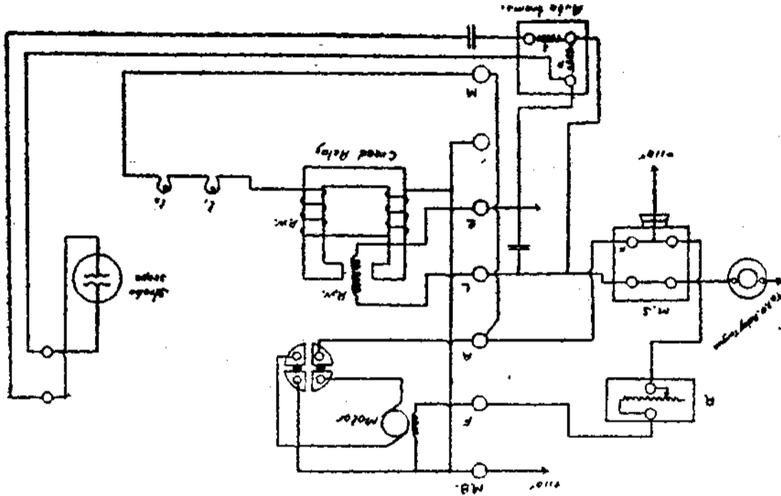
Creed Receiver Connections
