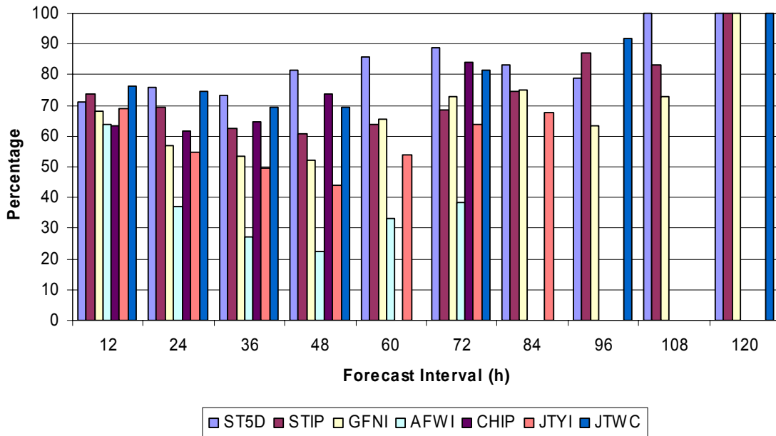
Figure 4.16 Percentage of Good intensity trends during the decay Phase III for the combined 2003 and 2004 seasons. Sample sizes of the verified forecasts range from 400 at 12 h to less than 30 by the 96-h point. A Good forecast during decay indicates that the magnitude of the forecast decay rate is within +/- 10 kt of the actual decay rate.
