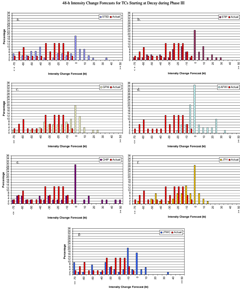
Figure 4.22 (a-g) Phase III graphs of actual 48-h intensity change distribution plotted with the 48-h intensity change distributions of all the various techniques and JTWC.
