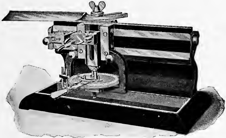
FIG. 105.—Large laboratory microtome (Bausch & Lomb).
