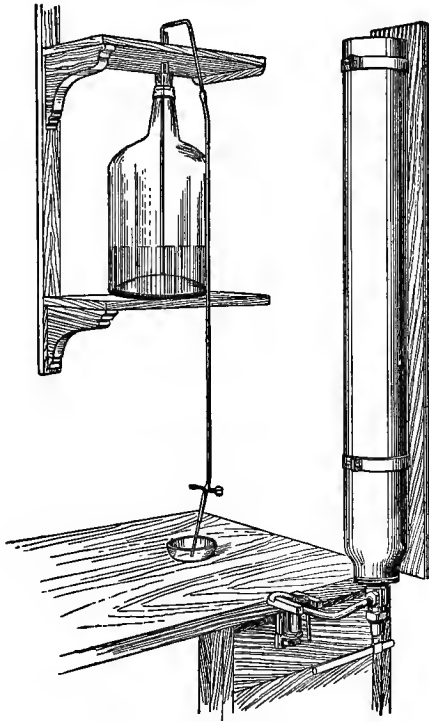
FIG. 103.—Freezing microtome.
