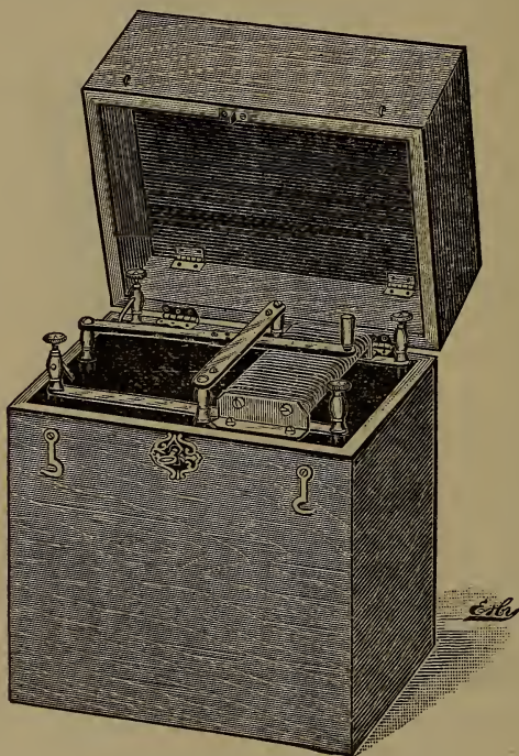
FIG. 133.—TRUAX STORAGE BATTERY.
