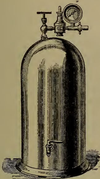
FIG. 21.—AIR-METER OF IMPROVED PATTERN.
