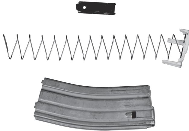
Figure 3-37. Magazine Disassembled.
