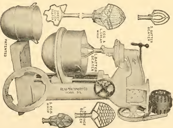
Type "D," 30 and 80-Quart bowls
