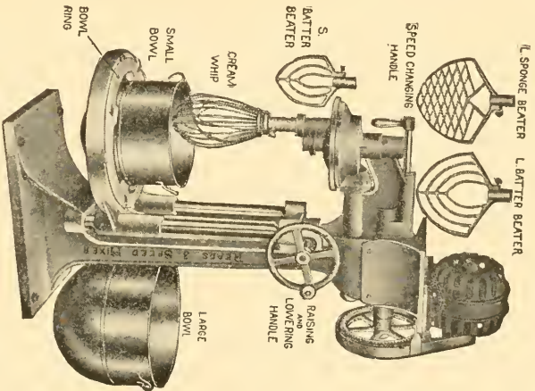
Type "B," 30 and 80-Qt. bowls
