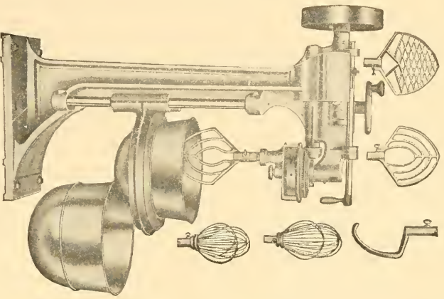
Type "A," 30 and 60-Qt. bowls
