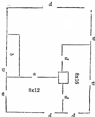
Bee House.
