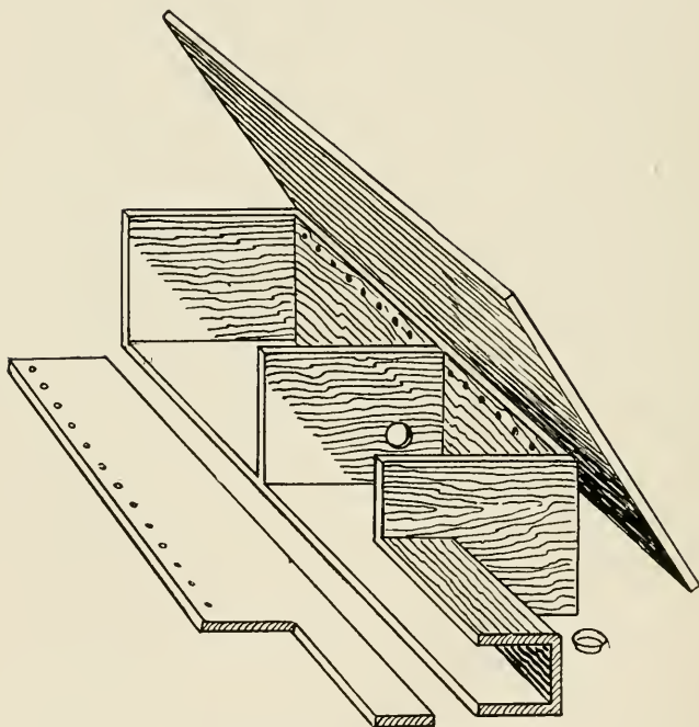
Construction of Nest Box (Side Removed)
