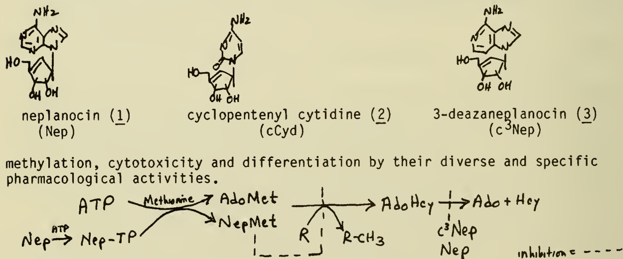
Fig. 1. Sites of action of neplanocin (Nep) and 3-deazaneplanocin ( c^3Nep )
