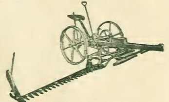
Avery 5 ft. Champion Mower.
