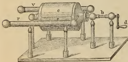
Cylinder-Elektrifiermaschine.
