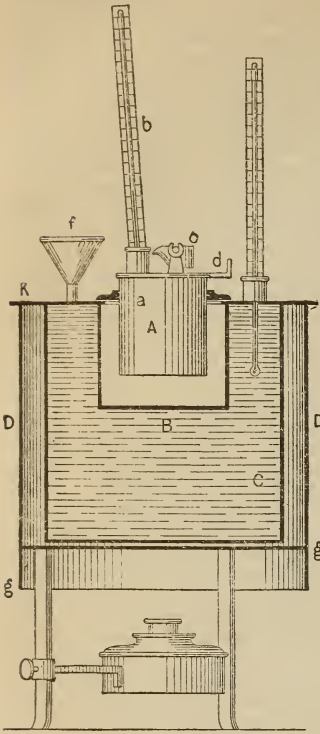
Abelscher Petroleumprober.
