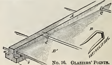
No. 16. GLAZIERS' POINTS.
