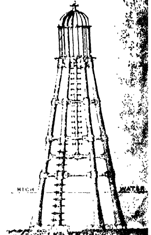
Fig. 1. Elevation of a First-class Cast-iron Beacon; total height above high water, 55 feet.
