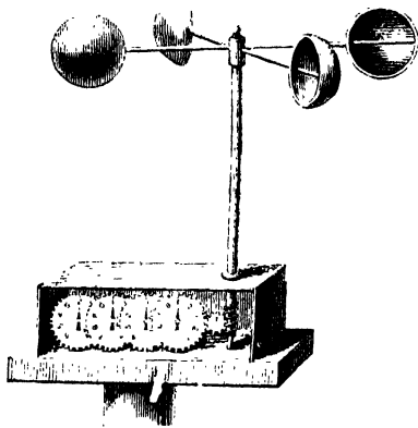
Robinson's Hemispherical-cup Anemometer.
