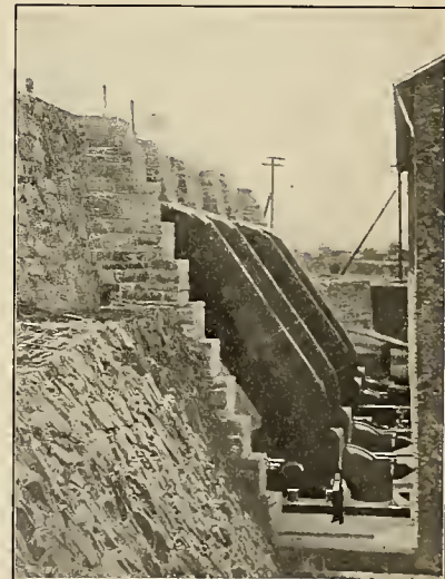
The Four Penstocks, through which the Water Plunges from the Forebay to the Power Wheels of the Folsom Power.
