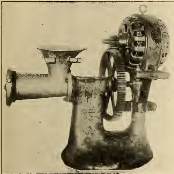
Motor Driven Meat Chopper.
