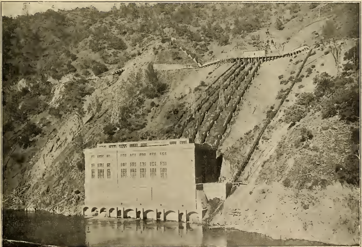
Power House, showing Transmission-line Towers, Pipe-lines and Surge-pipe, and Cable Crossing River.
