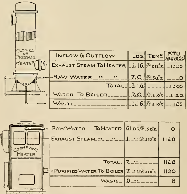
Fig. 2. Comparison of Open and Closed Heater.
