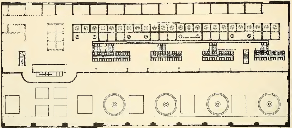
GALLERY PLAN EL. 57.5
