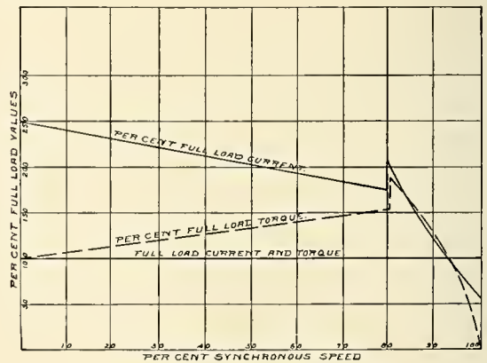
Speed—Torque—Current Curves.
