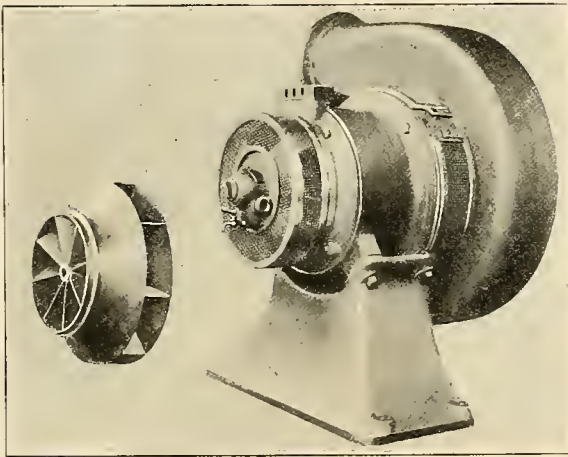
Union Iron Works Ventilating Set.
