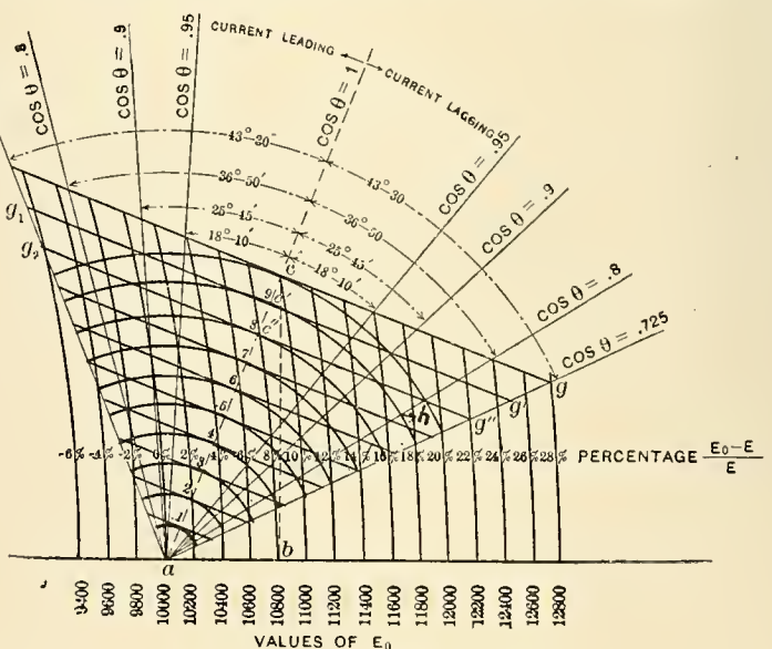
Fig. 2. Regulation of Transmission System.
