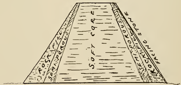
Former Construction.
