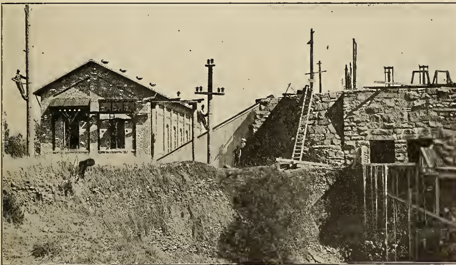
Folsom Power House and Granite Forebay.
