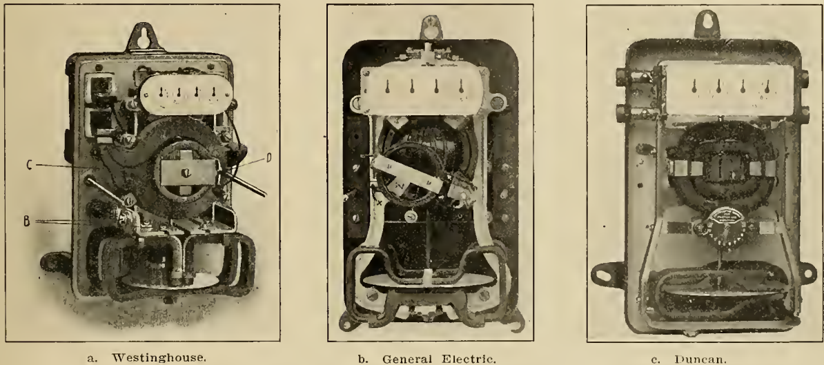
Fig. 45.—Types of Commutating Meters.
