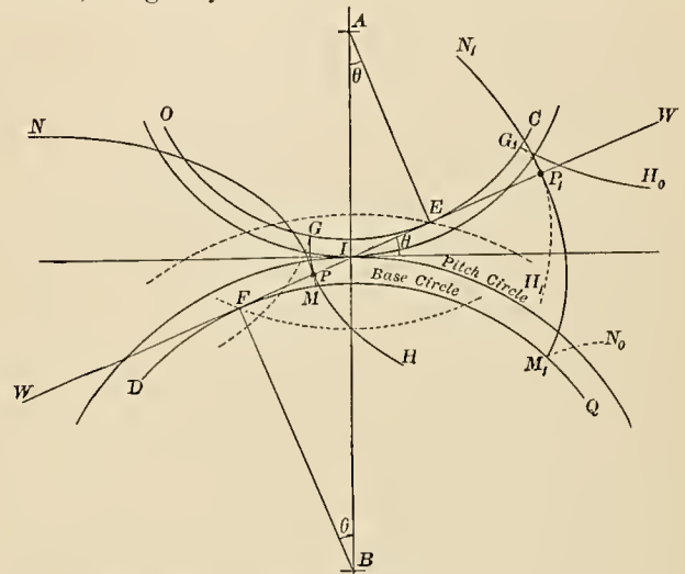
From LeConte's "Mechanics of Machinery," Fig. 15.
