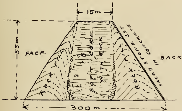
Amended Construction.
