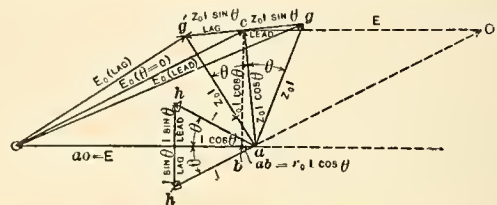
Fig. 9. Synchronous Motor Diagram.
