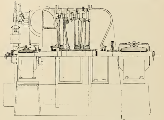
Assembly of 1000 k. w., 1500 r. p. m., low pressure horizontal Curtis steam turbine.
