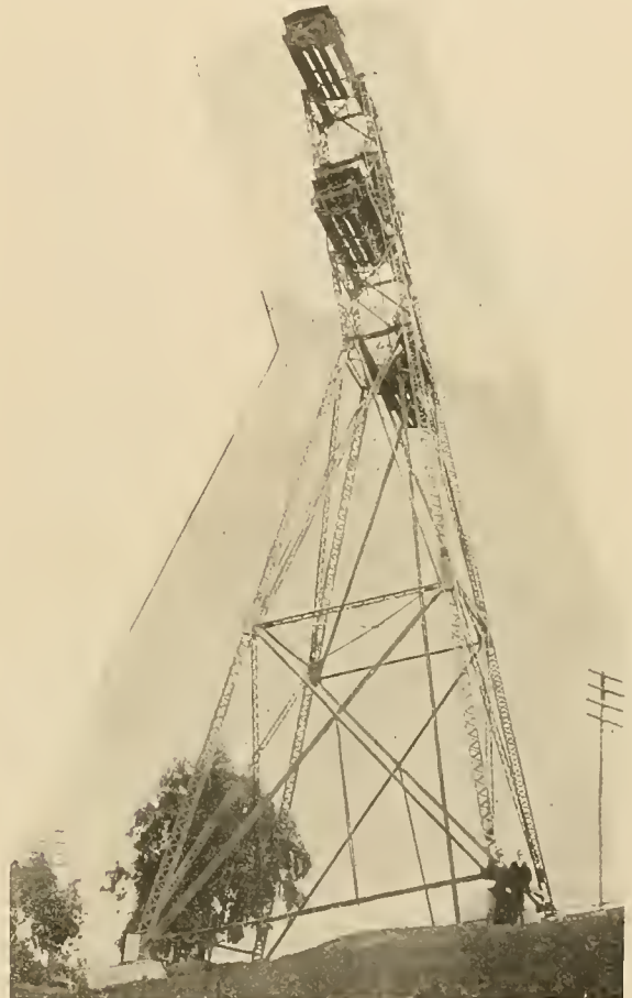
The Leaning or North Tower.
