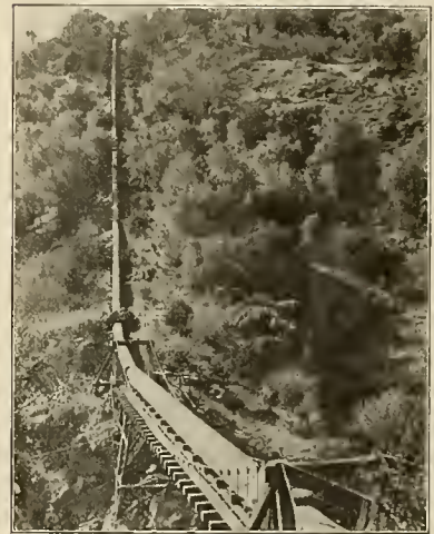
Inverted Syphon carrying Brown's Valley Ditch across Canyon below Yuba Power Plant.
