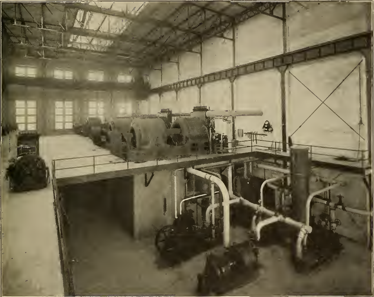
Steam Turbine Reserve at Oakland Station Great Western Power Co.
