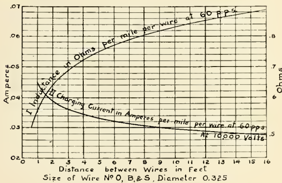
Fig. 7. Reactance and Charging Current per Mile.
