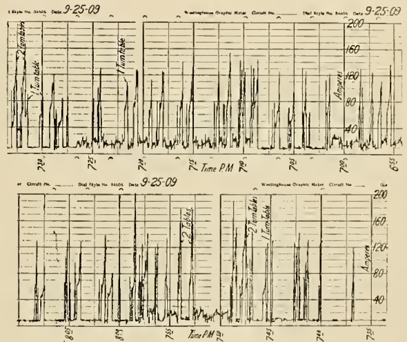
Graphic Meter Record of Motor Driven Locomotive Turntable Loads.
