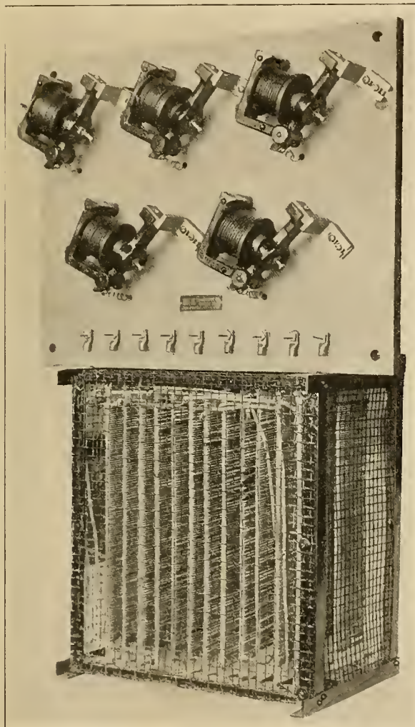
Regulator.
