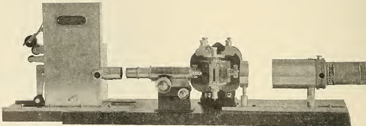
Fig. 4. Rapid Receiver.
