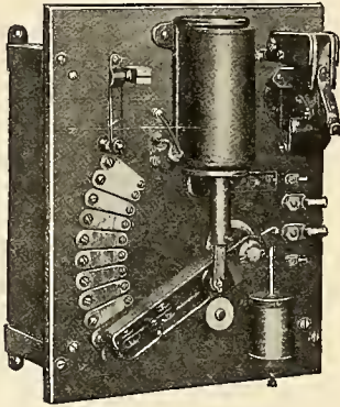
Fig. 1. General Electric Self-Starting Controller.
