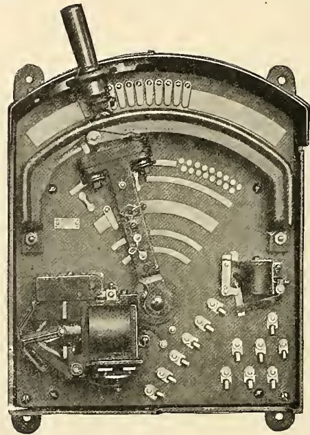
Printing Press Controller with Cover Removed.
