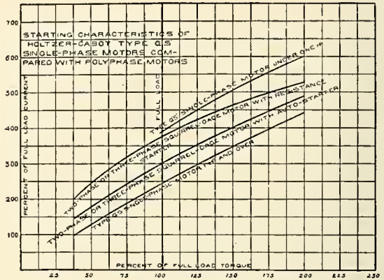
Comparative Starting Currents for Induction Motors.
