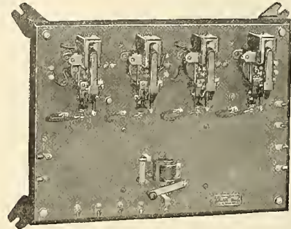
Fig. 3. Limit Switch of CR 130 Valve Controller.
