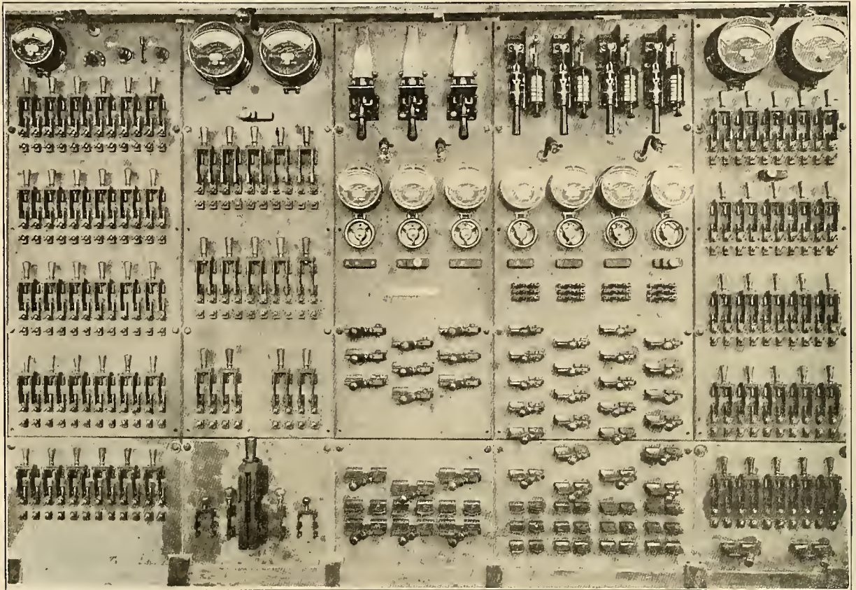
Main Switchboard.
