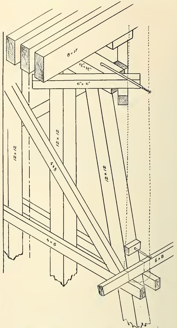
Standard Connection Between Pole and Trestle Bent.
