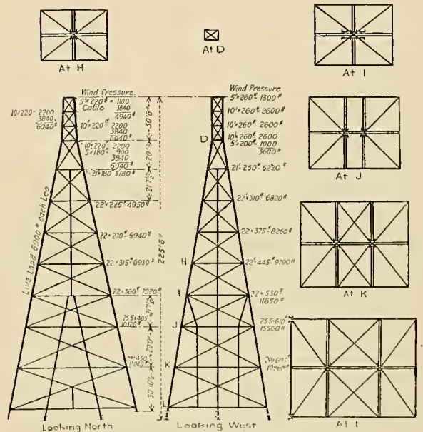
Stress Diagram of North Tower.
