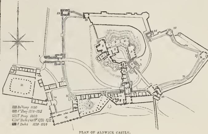
PLAN OF ALNWICK CASTLE.
