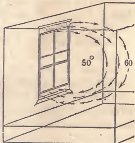
Conditions in which the air escapes below.
