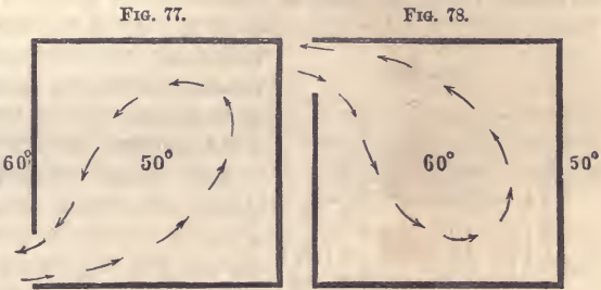
Conditions in which openings in rooms produce exchange of air.
