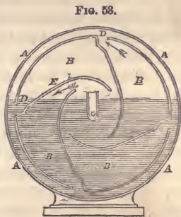
Meter for measuring the flow of Gas.
