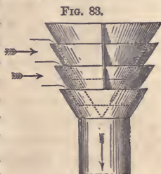
Emerson's Injector.
