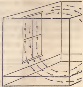
Currents produced in winter by single windows.
