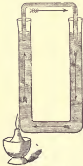
Circulation of water.
