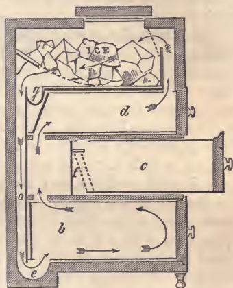
Lyman's Bureau Refrigerator.
