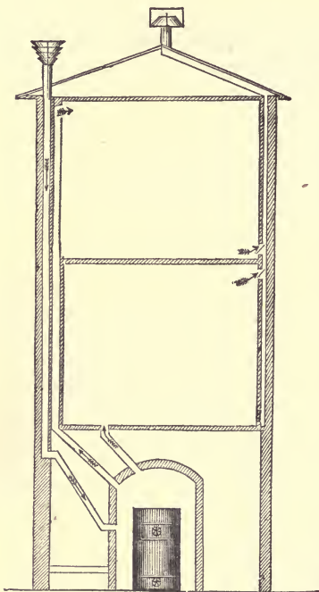
Manner of warming by Hot-Air Furnaces.
