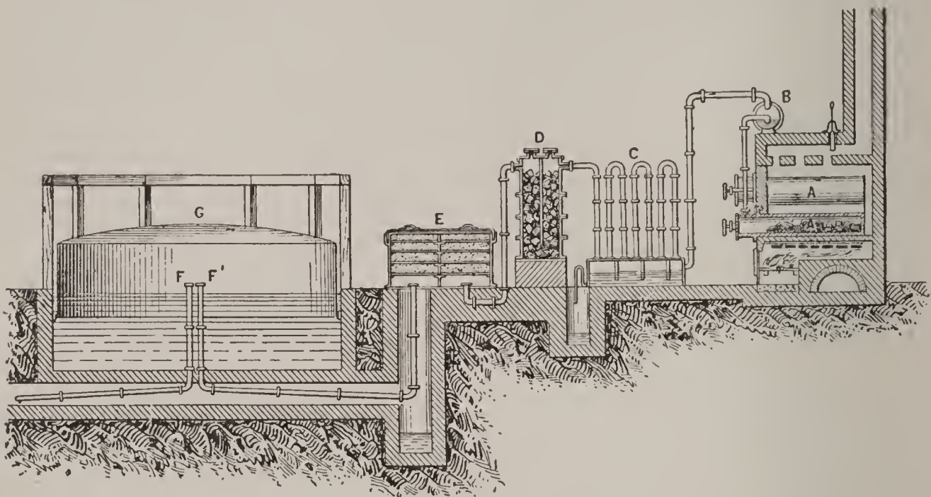
Gas-work, shown in section.
