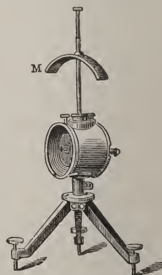
Fig. 4.—Mirror Galvanometer.
