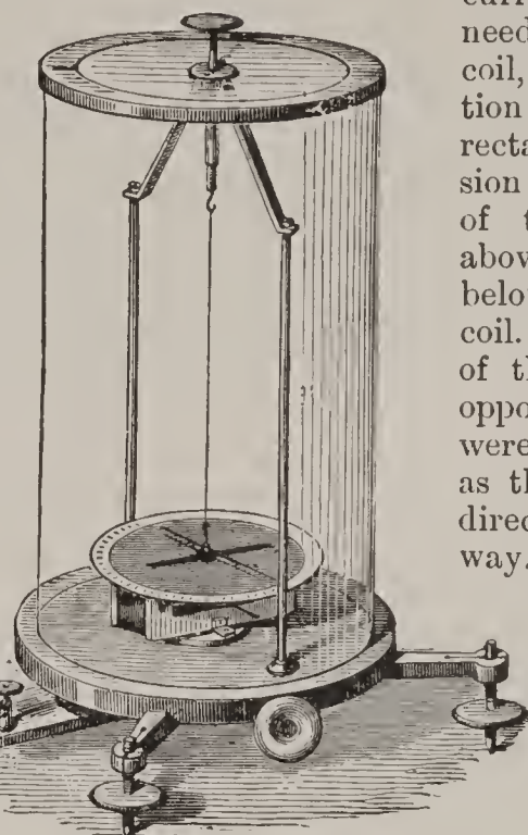
Fig. 1.—Astatic Galvanometer.
