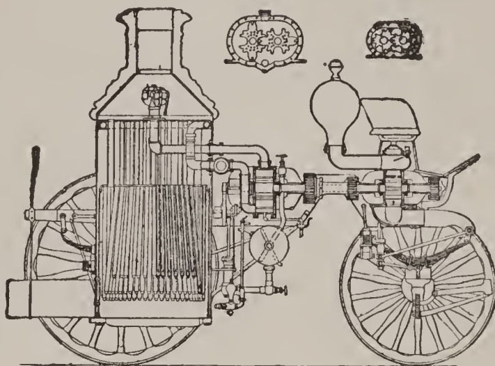
Vertical Section of Platform-spring Steam Fire-engine.
