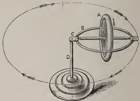
Gyroscope.
