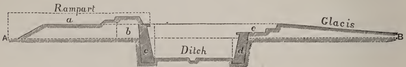
Section through line of Fortifications.
