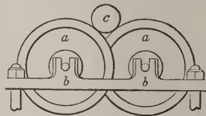
Friction-wheels.
