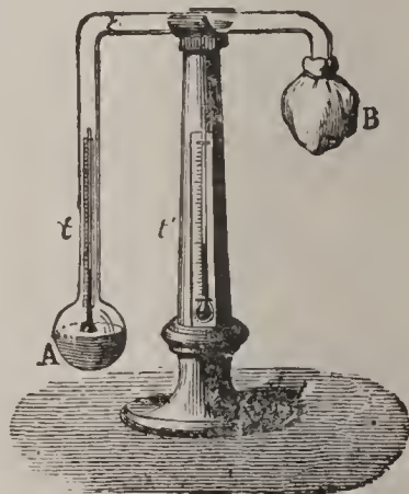
Daniell's Hygrometer.
