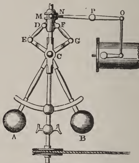
Governor of a Steam-engine.
