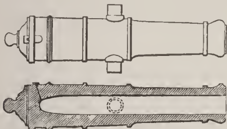
Brass Howitzer (24 pounder).
