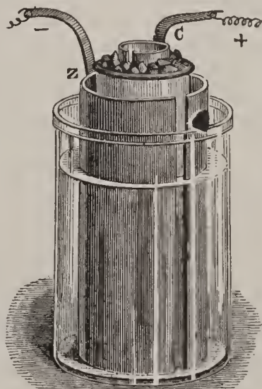
Fig. 3.—Daniell's Cell.
