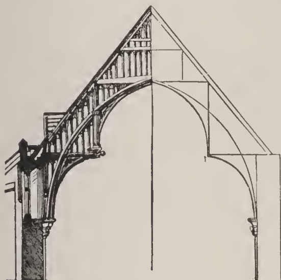
Hammer-beam Roof, Westminster Hall.
