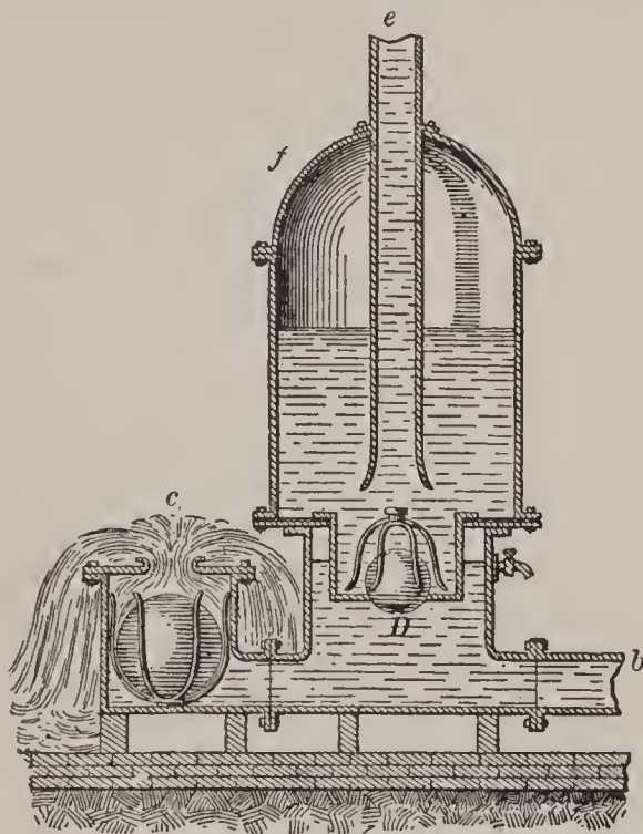
Hydraulic Ram.
