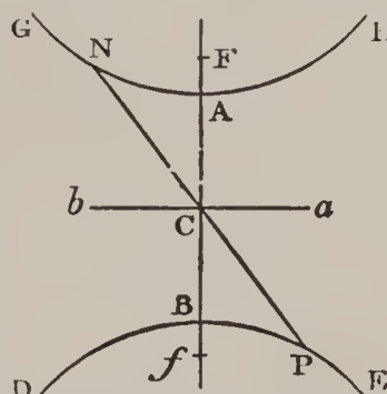
Hyperbola— D B E , G A H , are opposite hyperbolas; F , f , foci; C , centre; A B , transverse axis; a b , conjugate axis; N C P , a diameter.
