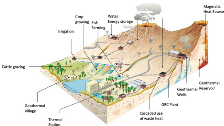
Fig. 19.17 Conceptual diagram of a geothermal village concept (Modified from Varet et al. 2014)
