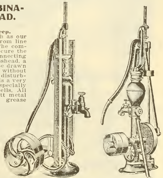
No. 1 Pump Jack. Fig. 1427—Pumping Head.
