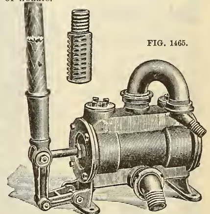
Fig. 1465—Pump with Strainer Hose Couplings and Clamps.....$7.00 1-inch Discharge Hose, per foot... .20 2-inch Suction Hose, per foot..... .40
