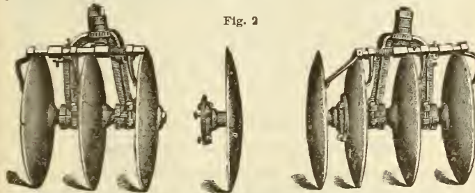
This cut shows the gangs with a fourth disc attachment and how easy it is for to convert the Janesville Disc Cultivator into a disc harrow.
