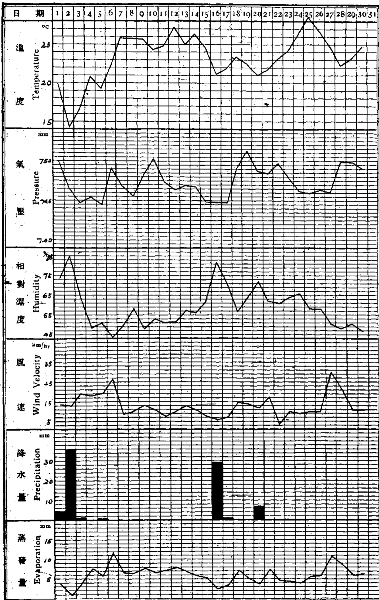
中華民國二十四年六月份各項氣象要素逐日變遷圖 March of Different Meteorological Elements in the Month of June, 1935.
