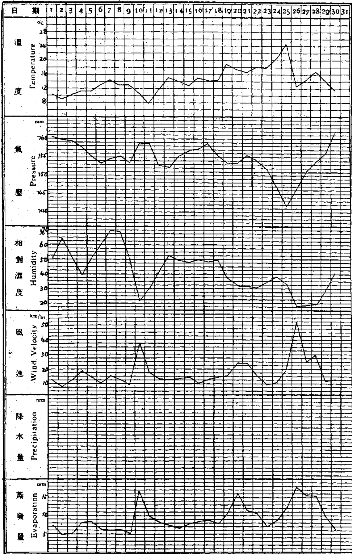
中華民國二十四年四月份各項氣象要素逐日變遷圖 March of Different Meteorological Elements in the Month of April, 1935.
