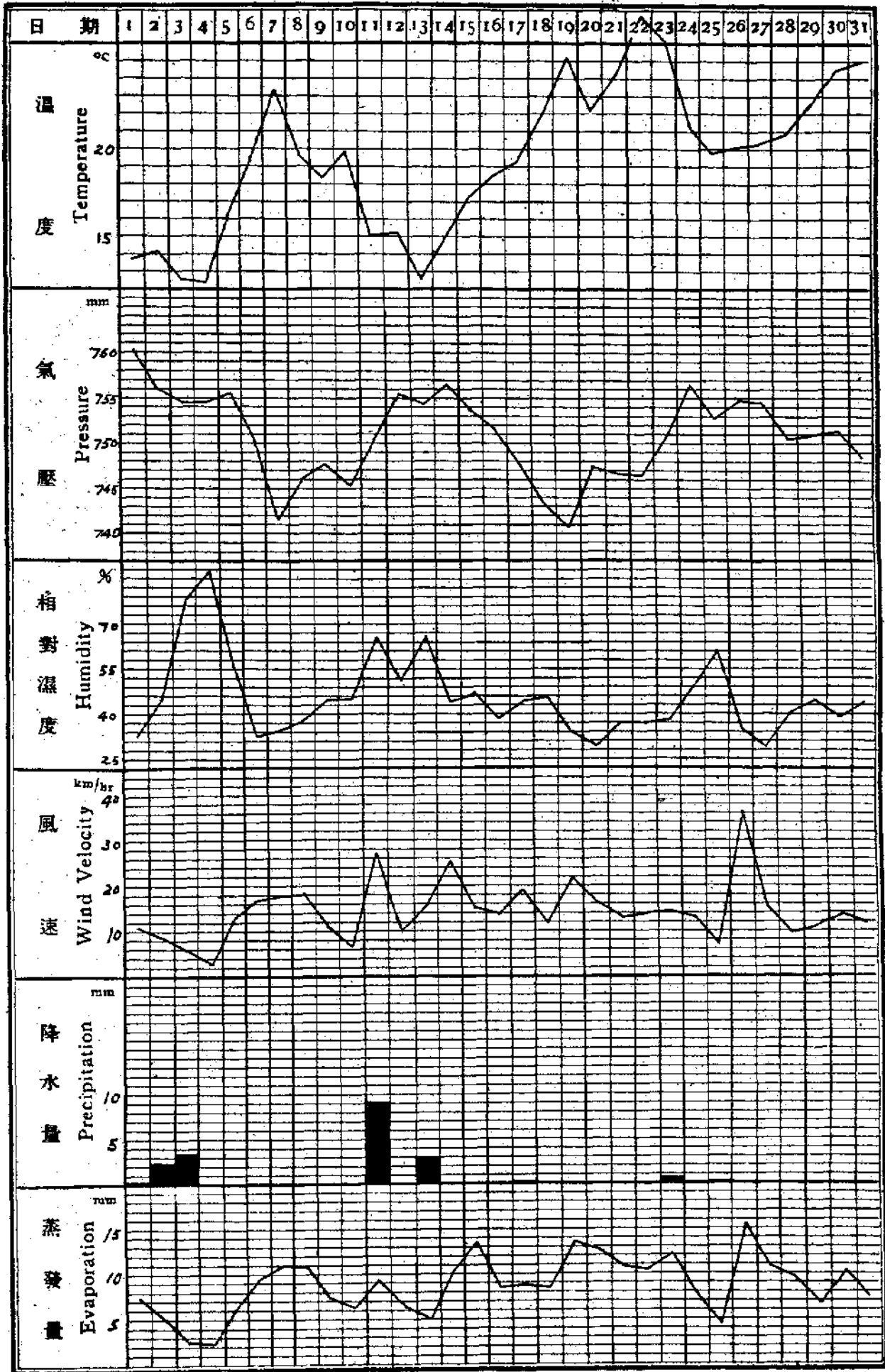
中華民國二十四年五月份各項氣象要素逐日變遷圖 March of Different Meteorological Elements in the Month of May, 1935.
