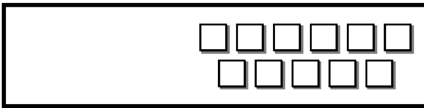
Figure 3.3: Struct pointing to 11 boxes, 4 filled with 0006, 7 the string "person"
