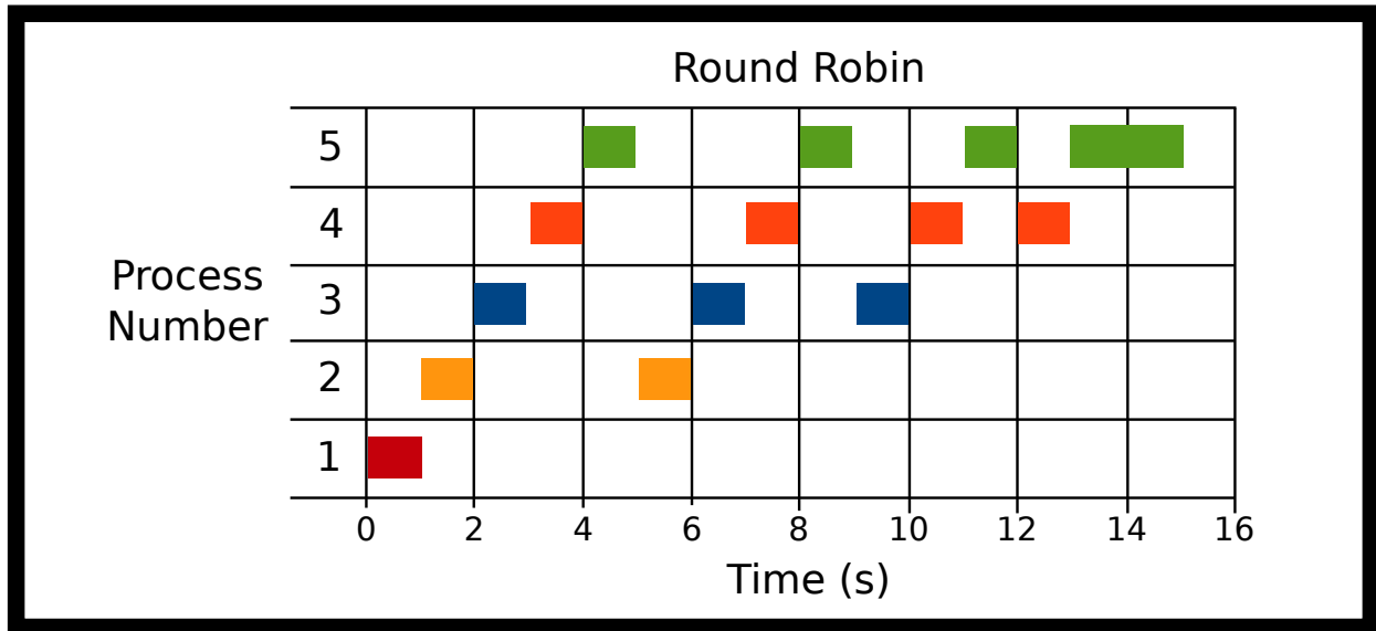
Figure 10.4: Round Robin Scheduling
