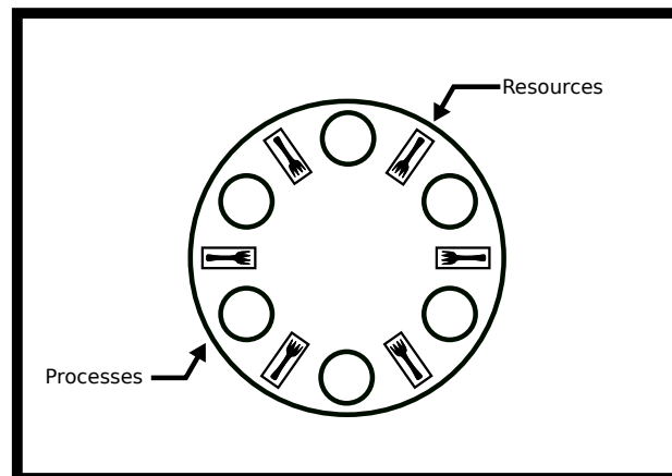
Figure 8.3: Dining Philosophers
