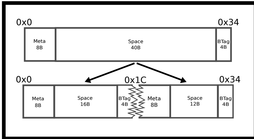
Figure 5.7: Malloc split
