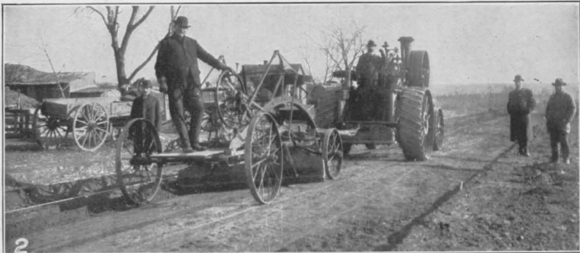
FIG. 2.—PREPARING SET GRADE FOR MACADAM ROAD WITH TRACTION ENGINE AND ROAD MACHINE, ARKANSAS CITY, KANS.
