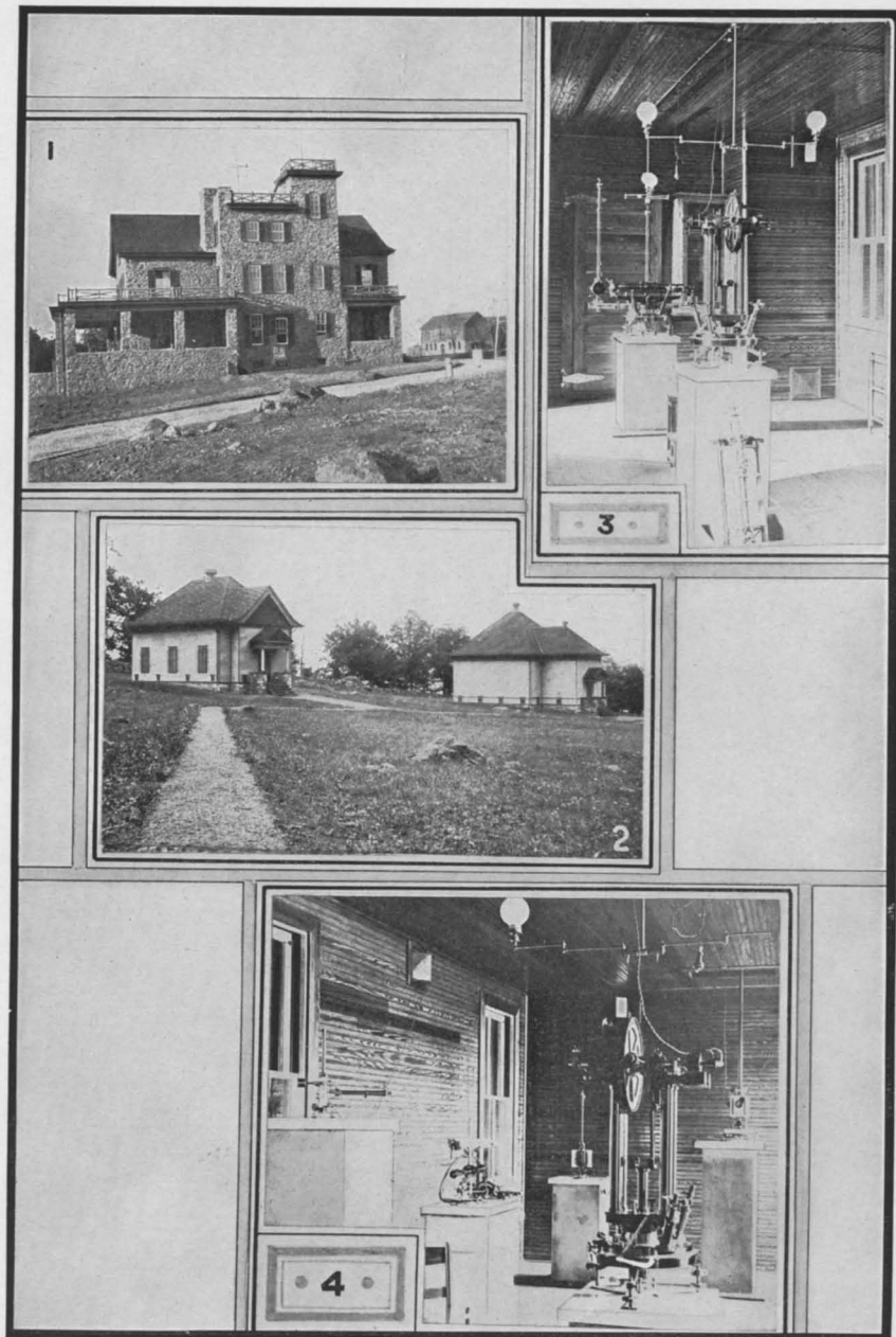
BUILDINGS AND INSTRUMENTS AT MOUNT WEATHER, VA.
