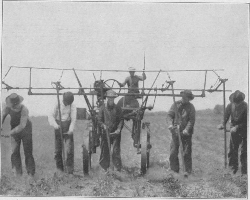
FIG. 1.—POWER HOE THAT MAY BE UTILIZED IN BLOCKING AND HOEING SUGAR BEETS.
