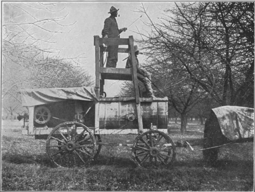
FIG. 2.—A GASOLINE POWER OUTFIT USED IN WESTERN NEW YORK. (ORIGINAL.)
