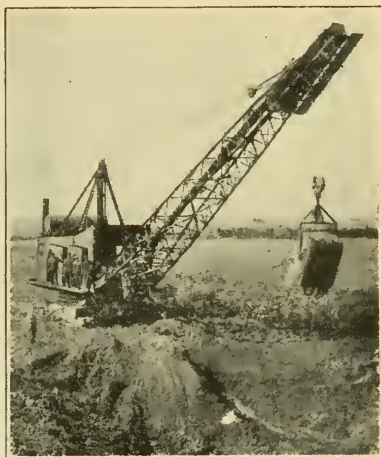
A type of mechanical excavator used in making open ditches.
