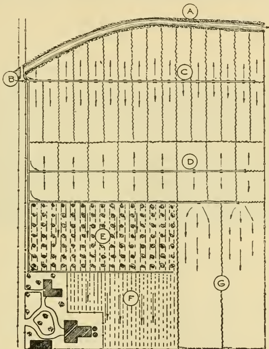
Sketch showing typical irrigation systems for a small farm. A, Irrigation canal. B, Farmer's head gate. C, Strip check system of irrigation. D, Square check system. E, Orchard irrigation by furrows. F, Furrow irrigation for field crops. G, Border irrigation.
