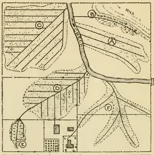
Plan of typical drainage system for a 160-acre farm. A , Single-line system of drainage. B , Cut-off drain to intercept seep water from the hill. C , Gridiron system of drainage for flat land. D , Herringbone system of drainage. E , Drainage of a pond. F , Natural system of drainage; also note the drain to the farm buildings.
