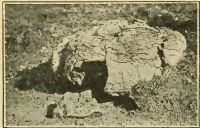
A rock that is being broken up to form soil, by the action of water, heat, and cold.
