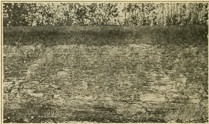
A soil that remained where it was formed. Observe the ledge of rock below the soil. It was from similar rock that the soil above was formed.
