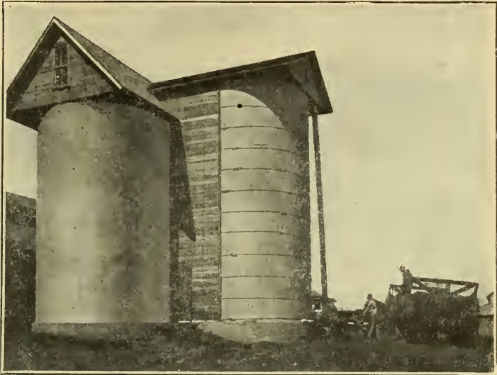
Filling a silo. A blower is used to elevate the material from the cutter to the silo.
