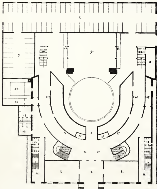
Plan Begane Grond.
