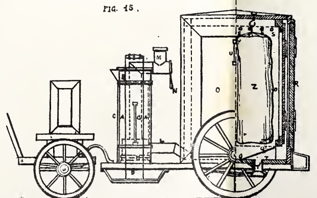
THURSFIELD'S AËRO-STEAM DISINFECTOR.
