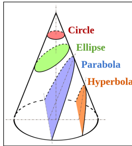
Figure 6. Conic sections (from S.A, n.d.)
