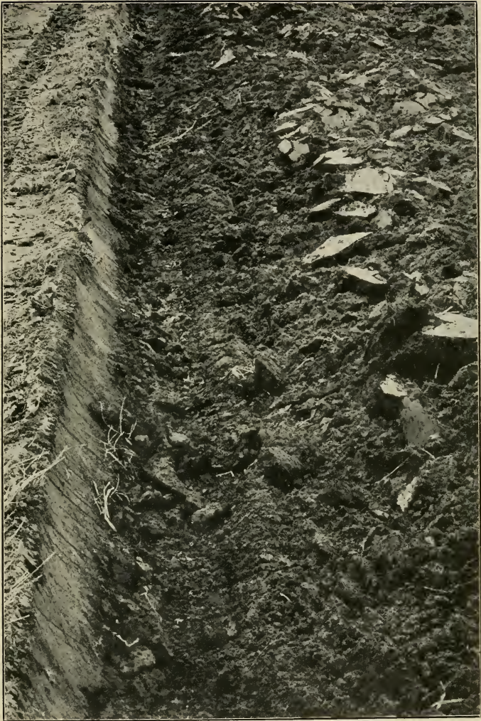
Notice the curved furrow wall and bottom and the way the earth is delivered as a turned furrow. It is entirely different from that of a mouldboard plow.
