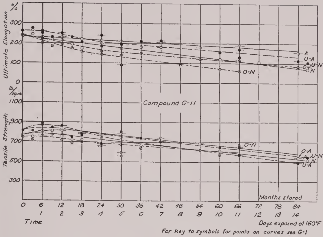
FIG. 16.—Tensile curves for compound G-II
