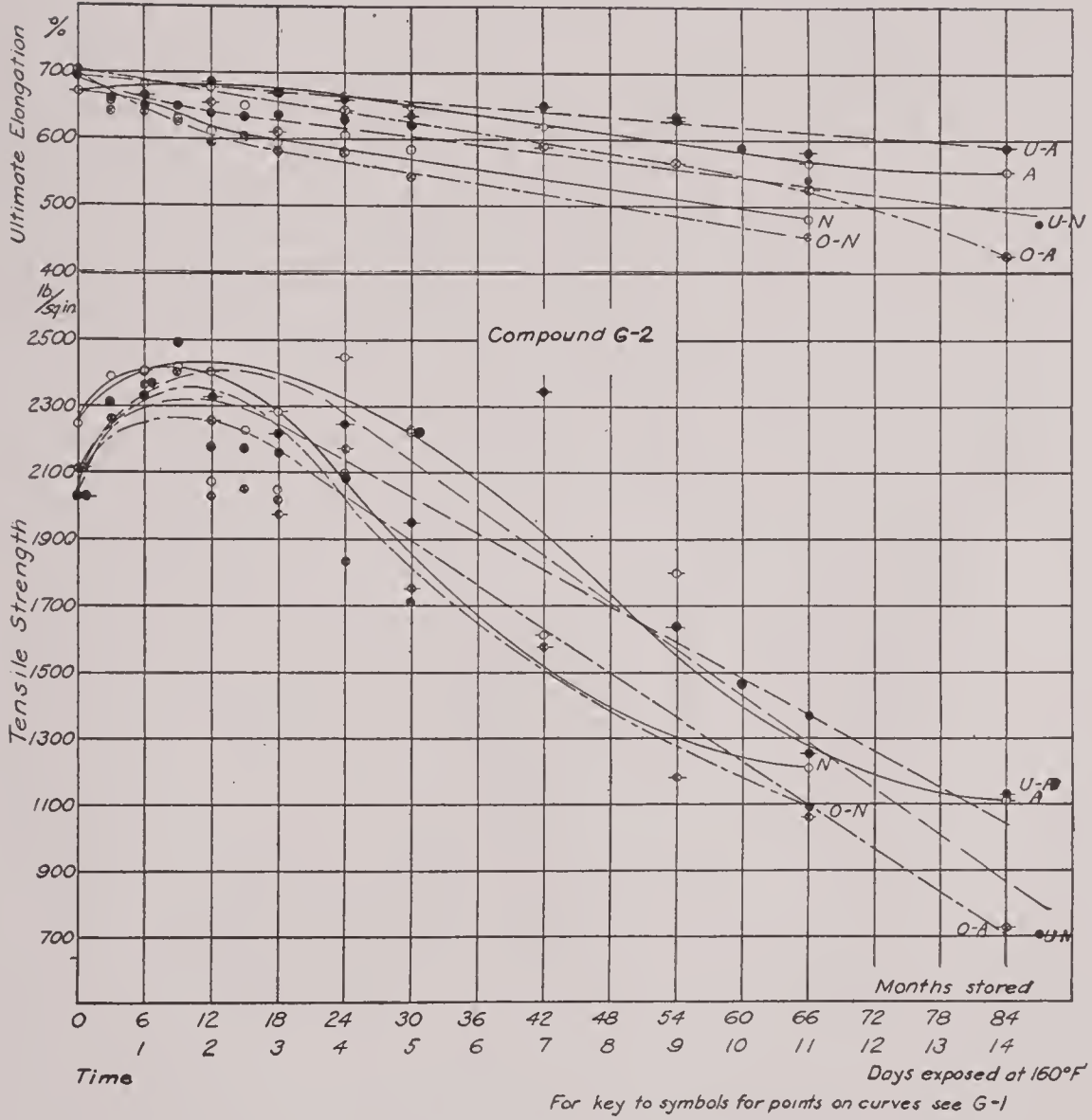
FIG. 7.—Tensile curves for compound G-2
