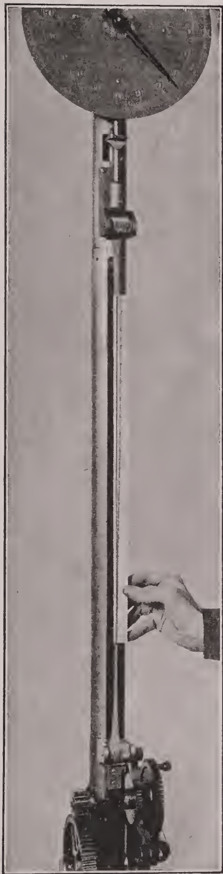
FIG. 27.—Illustrating method of measuring ultimate elongation
