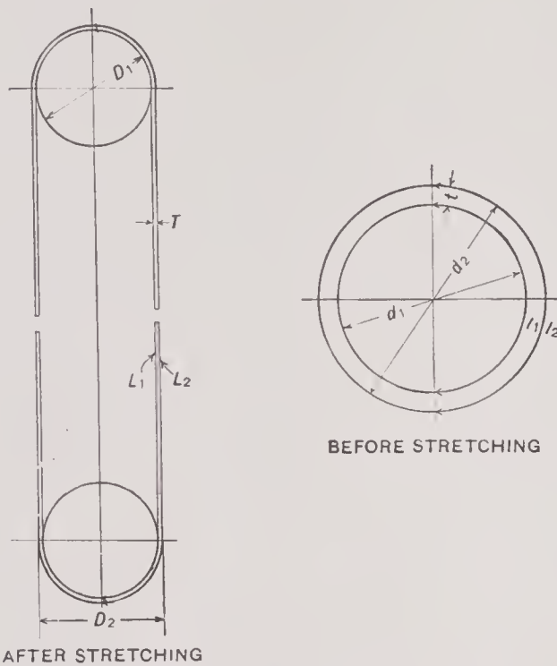
FIG. 33.—Ring test piece before and after being stretched
