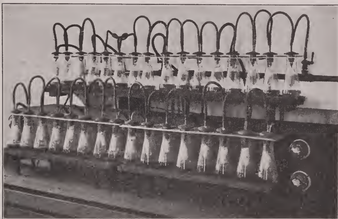
FIG. 47.—Acetone and chloroform extraction apparatus
