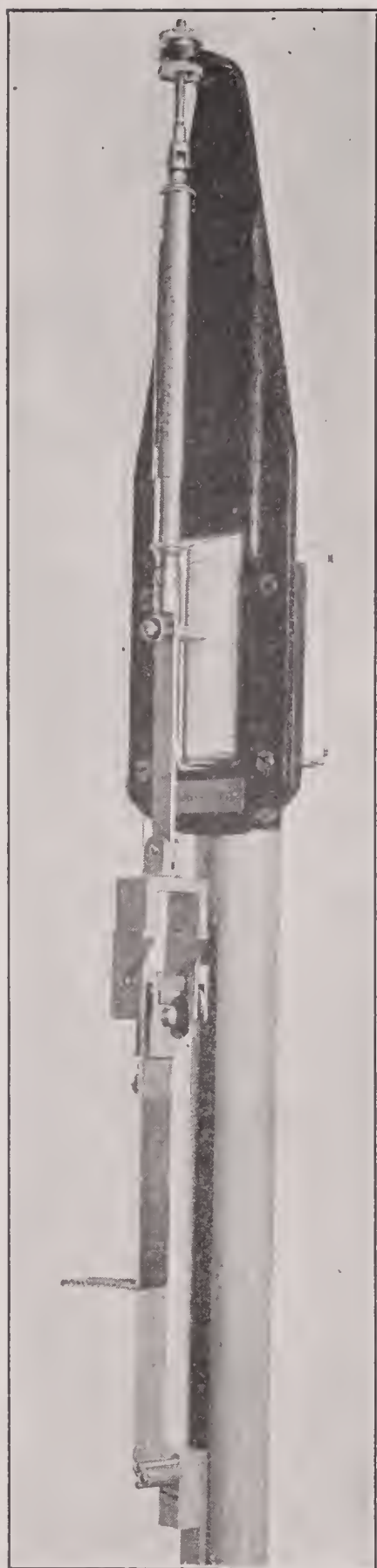
FIG. 37.—Autographic friction machine for measuring and recording the adhesion between plies of fabric
