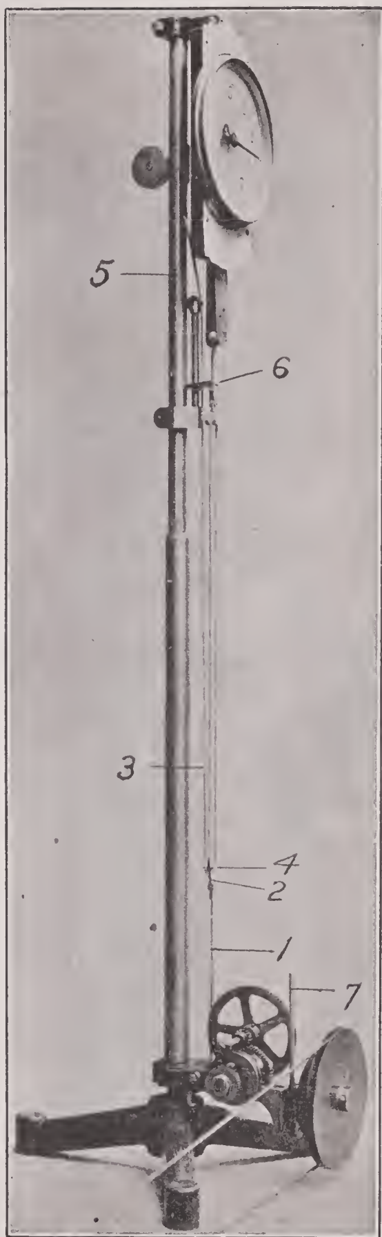
FIG. 29.—Motor-driven machine for testing rubber bands
