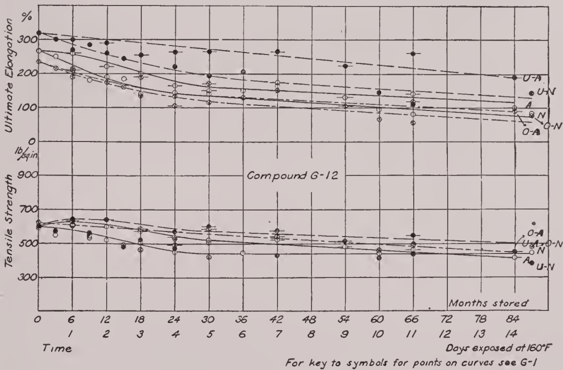
FIG. 17.—Tensile curves for compound G-12
