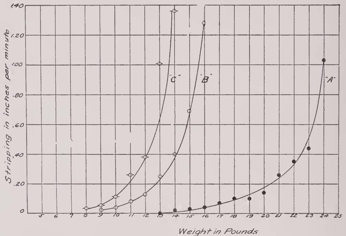
FIG. 41.—Friction test of rubber belting
