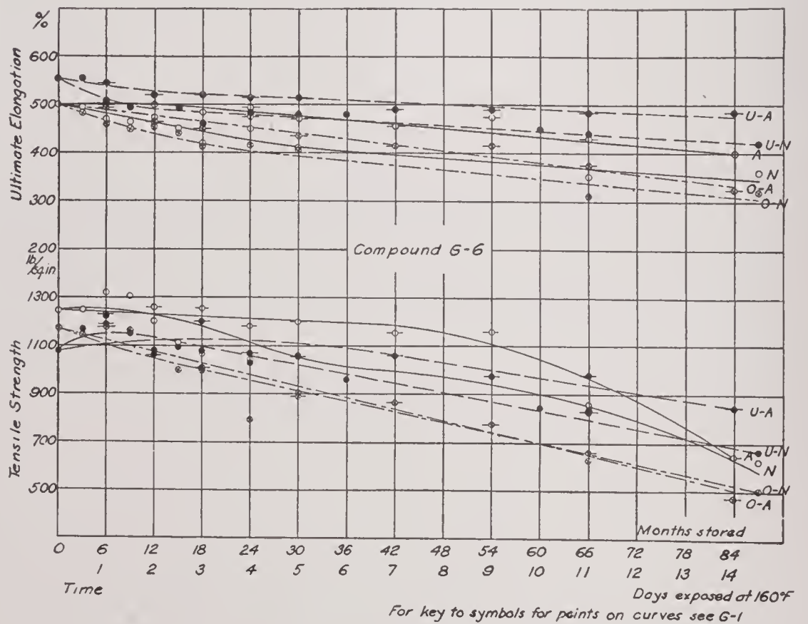
FIG. 11.—Tensile curves for compound G-6
