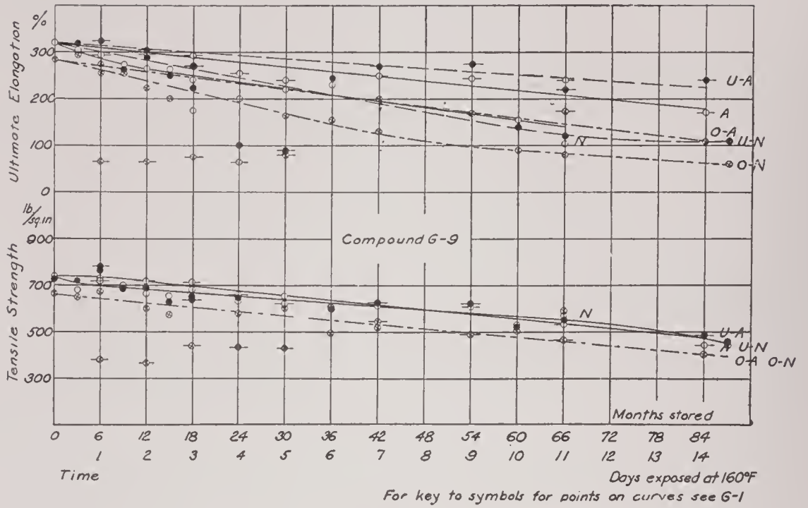
FIG. 14.—Tensile curves for compound G-9
