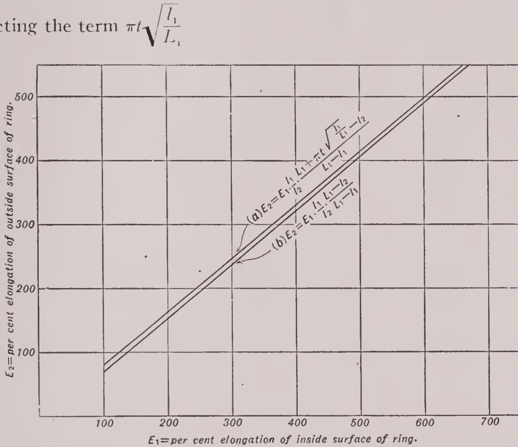
FIG. 34.—Relation between the elongation at the inside and outside of a ring
