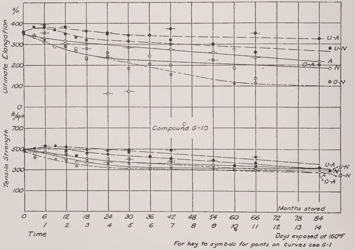
FIG. 15.—Tensile curves for compound G-10
