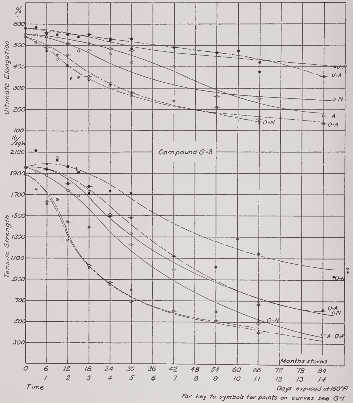
FIG. 8.—Tensile curves for compound G-3
