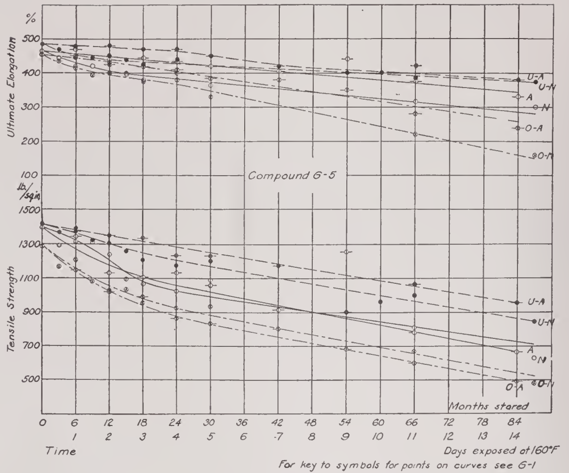
FIG. 10.—Tensile curves for compound G-5
