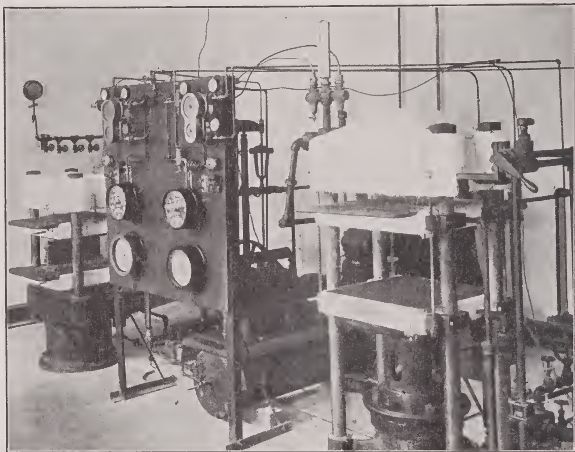
FIG. 4.—Vulcanizing press equipped with constant temperature control
