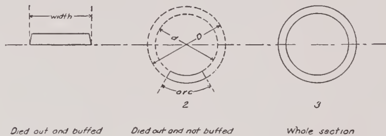
FIG. 45.—Cross section of test pieces
