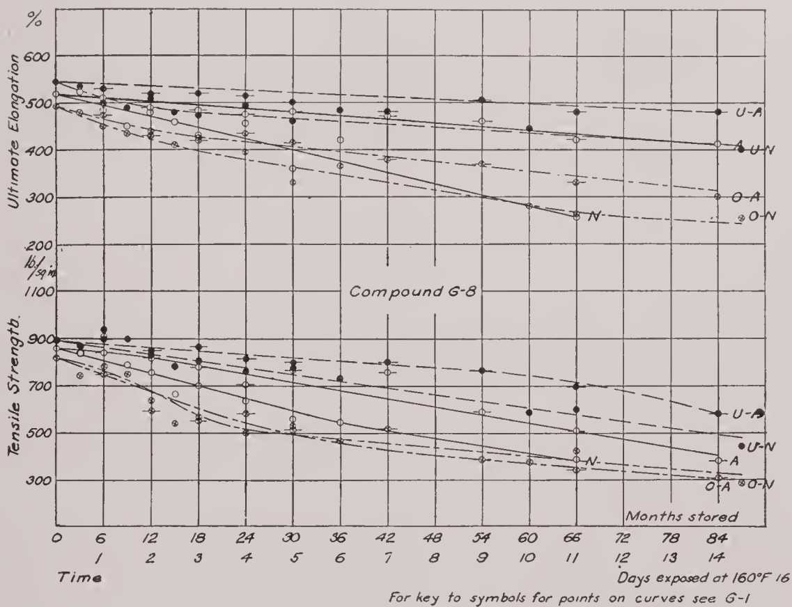
FIG. 13.—Tensile curves for compound G-8
