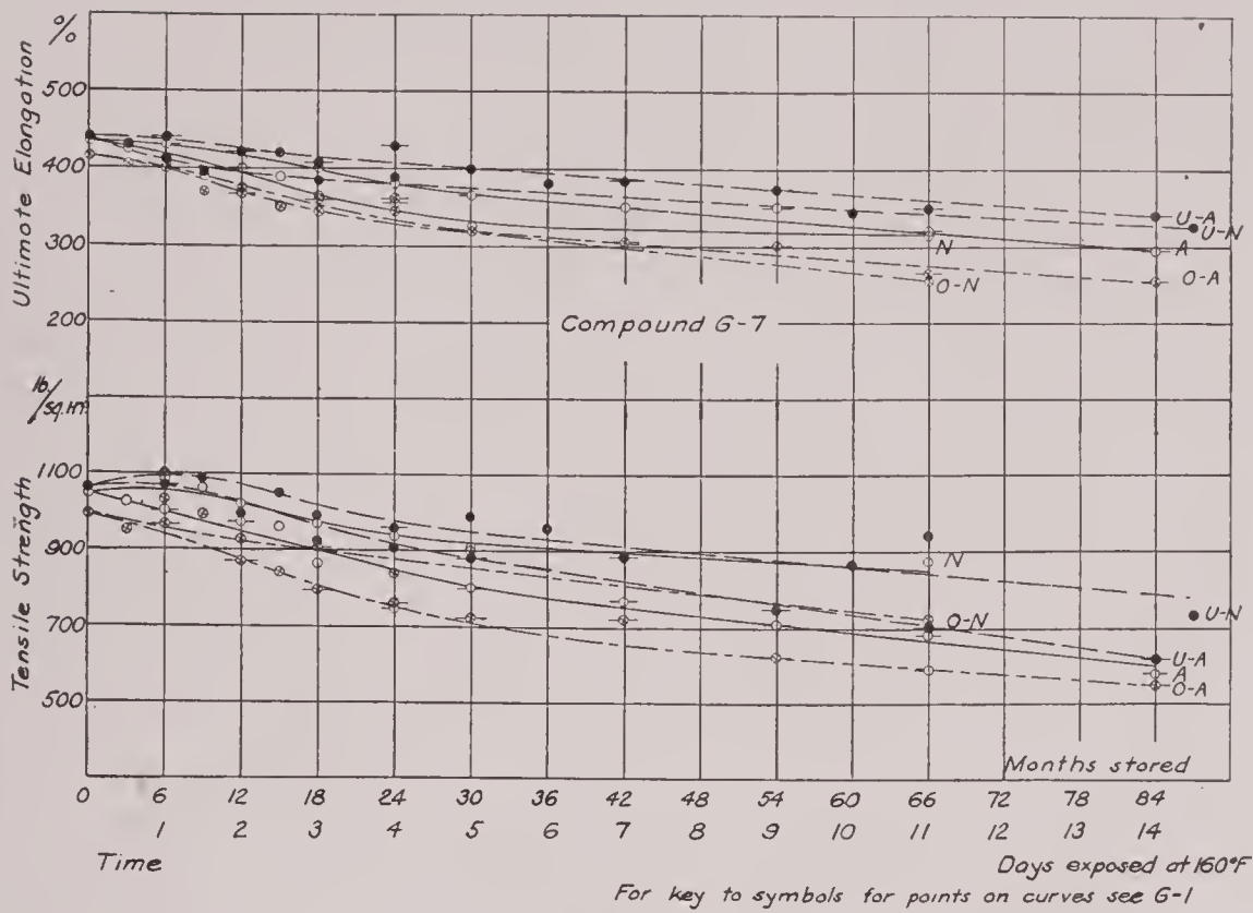
FIG. 12.—Tensile curves for compound G-7
