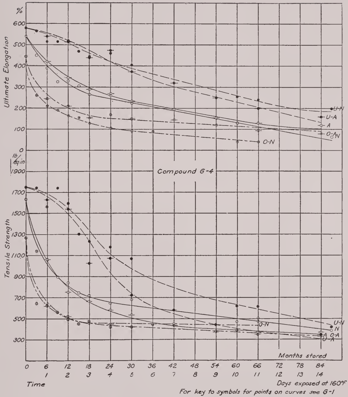
FIG. 9.—Tensile curves for compound G-4
