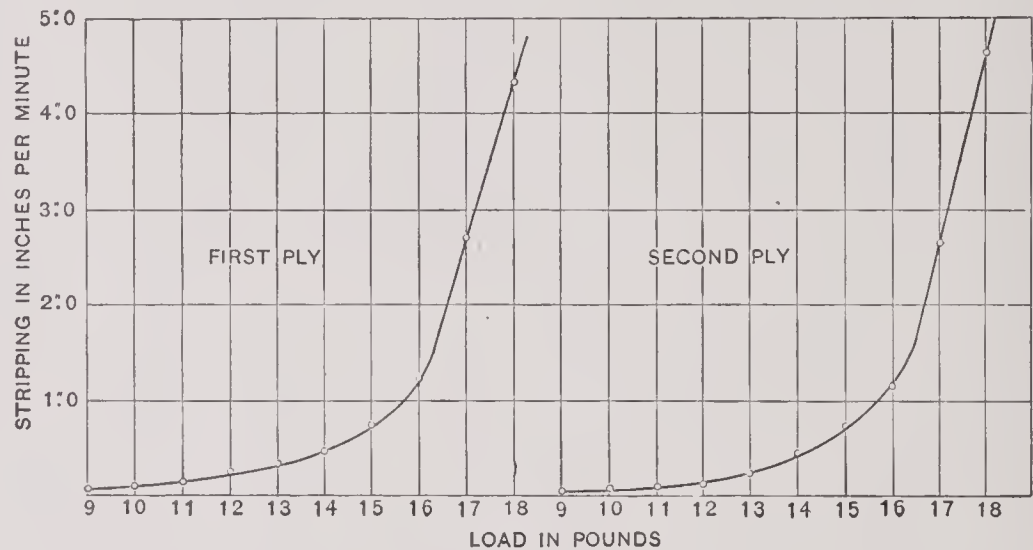
FIG. 39.—“Friction” test of rubber hose. Curves showing rate of stripping under different loads
