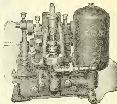
Fig. 1705—Power Sprayer with Automatic Governor.
