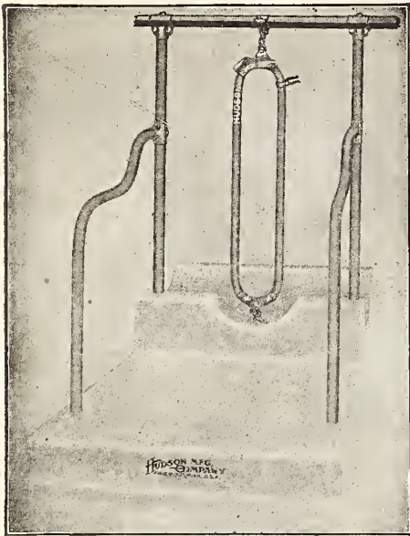
No. 1A66 Stall. No. 1A66—One Post Stall, with No. 66 Tubular Steel Stanchion. Price, $10.00 No. 1A5—One Post Stall, with No. 5 Wood Lined Steel Stanchion. Price, $10.25
