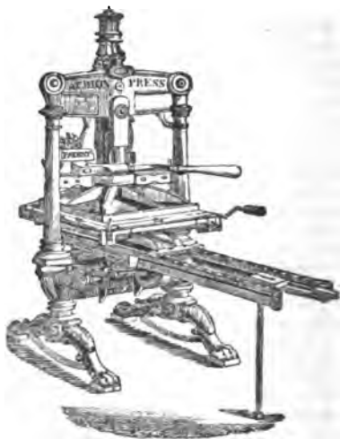
Dar. 408.—ALBION PRESS.
