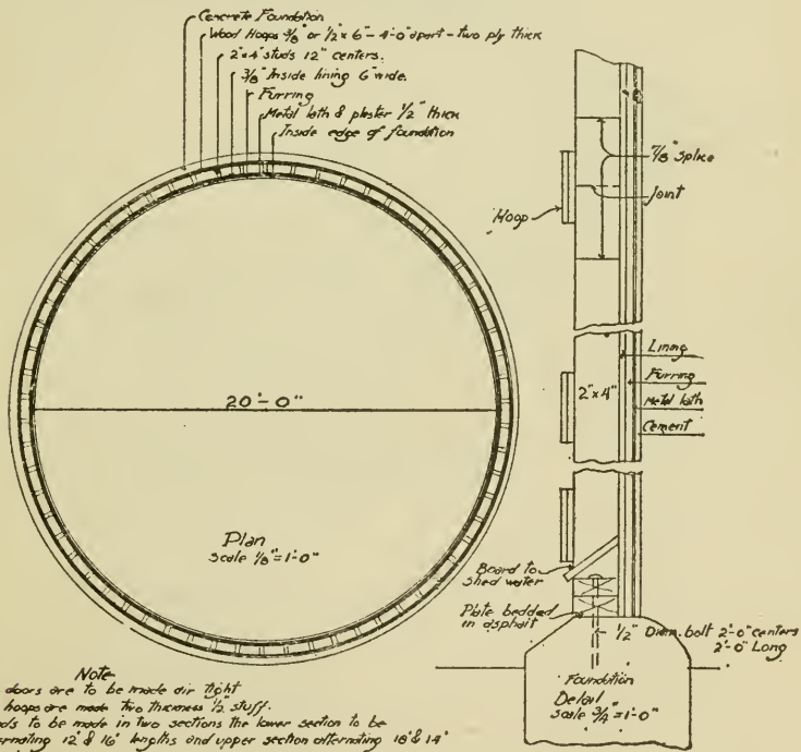
Fig. 10. Foundation plan and section of plastered round wooden silo.
