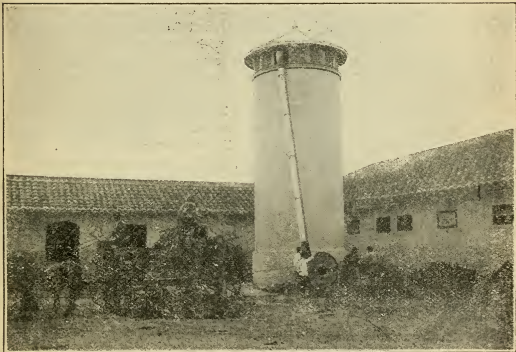
Fig. 28. Large cement silo and barns at Posto Zootechnico Central (Experiment Station) at Sao Paulo, Brazil, South America. Silo being filled with No. 17 Ohio Blower Machine.
