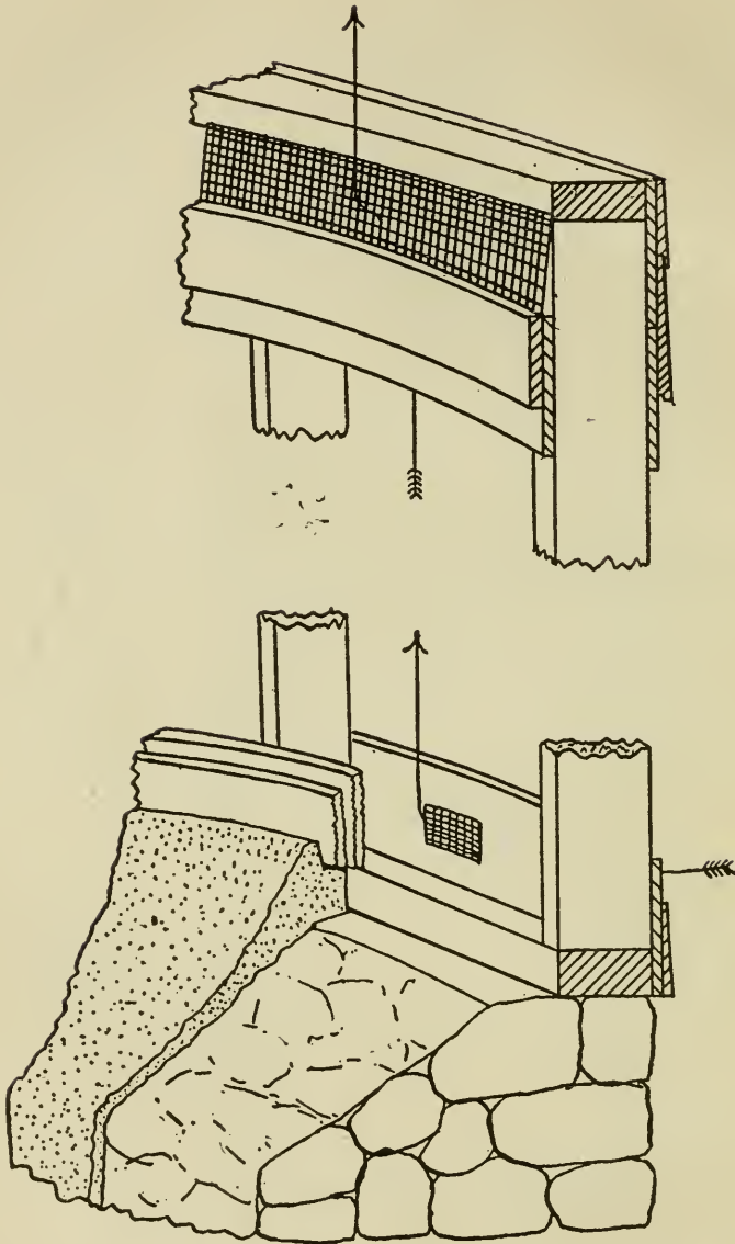
Fig. 3. Showing method of construction for ventilating the spaces between the studding in all-wood and lathed-and-plastered silos.
