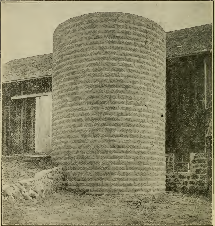
Fig. 42. Cement block silo. The kind built by Mr. Dunlap of Centre, Ralls county, Mo.—Courtesy Hoard's Dairyman.
