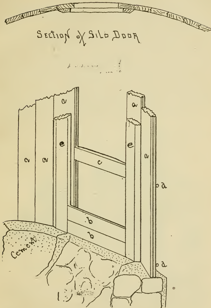
Fig. 17. a, a , Staves. b, b , Door Boards. c , Brace 2\frac{1}{2} by 6, set in. d, d , Hoops. e, e , Jamb Pieces.
