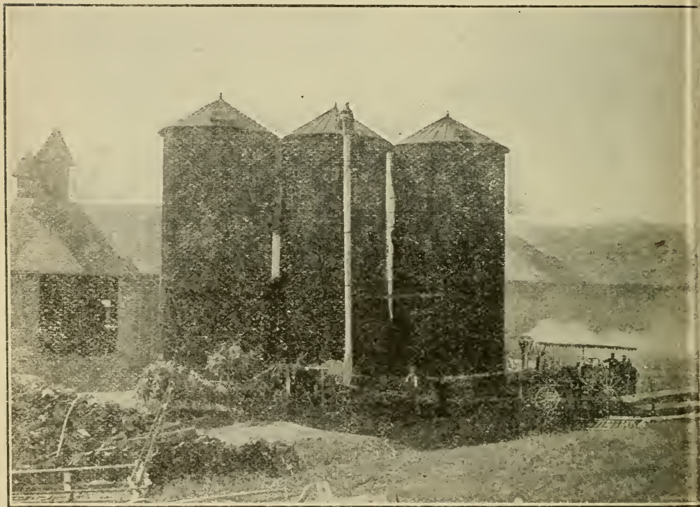
Fig. 29. This illustration shows a No. 19 Monarch Self-Feed Blower Cutter filling three forty-foot silos, 500 tons capacity, at the Ingleside Farms, Thorndale, Chester county, Pa. At the time the photograph was taken, this machine had just replaced an exploded fly-wheel cutter which nearly killed one of the workmen.
