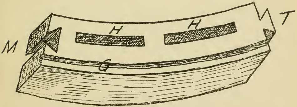
Fig. 39. Illustrates a type of concrete block used in silo construction. H. H. are holes left in blocks. T. and M. are dove-tailed tenon and mortise so made that blocks interlock when laid on the wall. G. is a groove made in block to imbed iron rod for reinforcing the wall.
