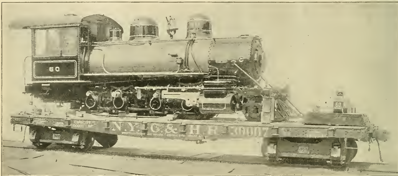
Narrow Gauge Locomotive for Interoceanic Railway of Mexico, Shipped on Fox Steel Car
