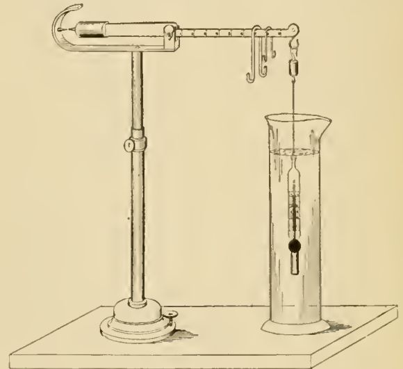
The Westphal Balance.
