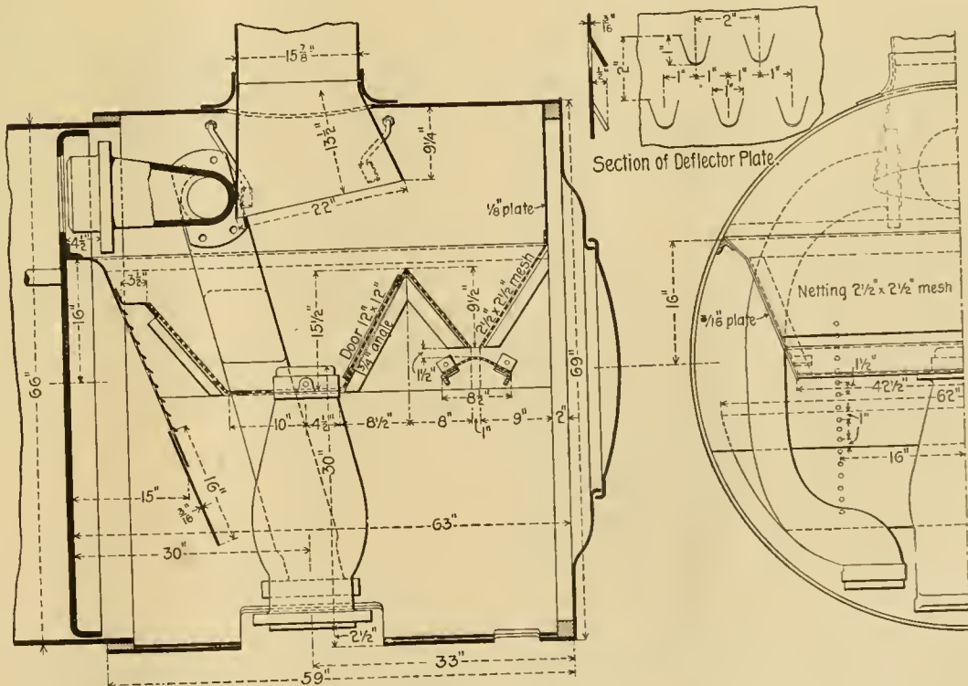
Fig. 6.—Wisconsin Central.
