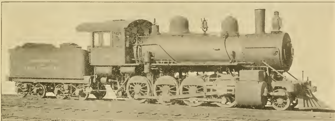
Schenectady Compound Consolidation Locomotive for the Ogdensburg & Lake Champlain Railroad.
