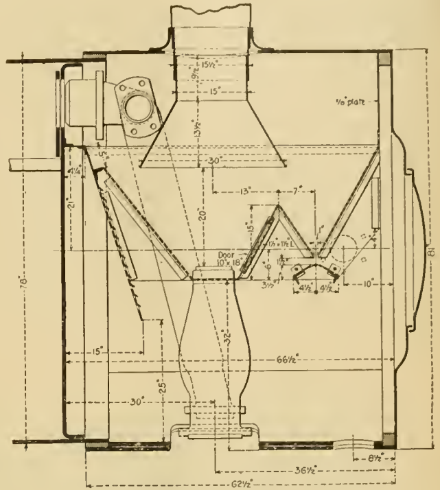
Fig. 5.—Great Northern.
