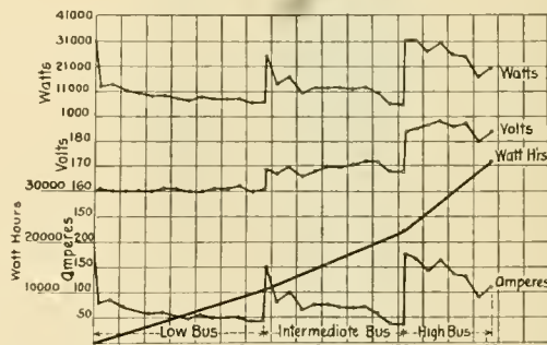
Fig. 3—Charges of Storage Battery Cells.
