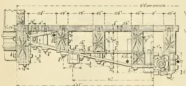
Section Showing Body Bolster.
