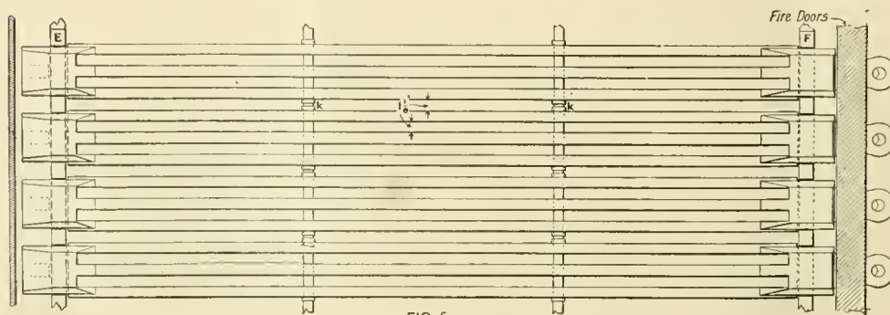
Figs. 3, 4 and 5.—Grates, Winans' Camel Engines.
