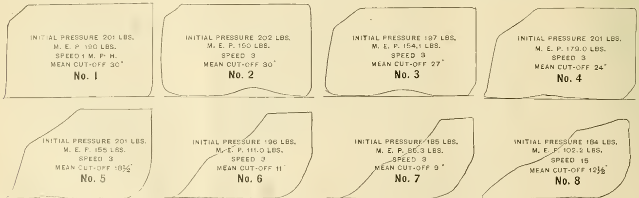
Indicator Cards—Great Northern Mastodon Locomotive.
