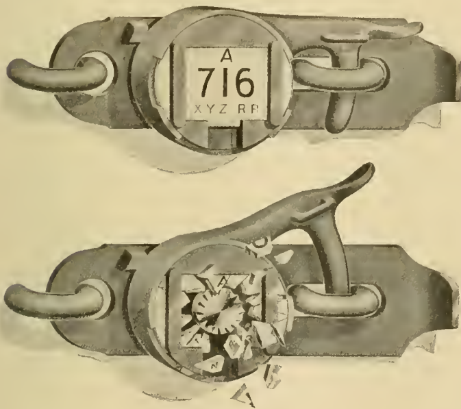
Wood's Car Seal.
