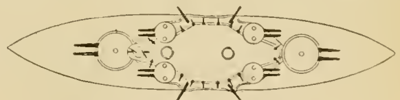
Gun Plan of the "Indiana."
