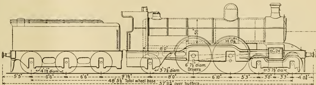
"Atlantic Type" Locomotive, Great Northern Railway, England.
