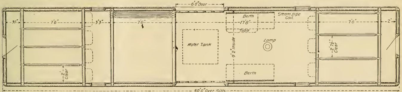
Car for Transporting Horses—C. & N. W. Railway.
