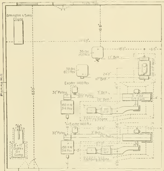
Engine and Dynamo Locations.
