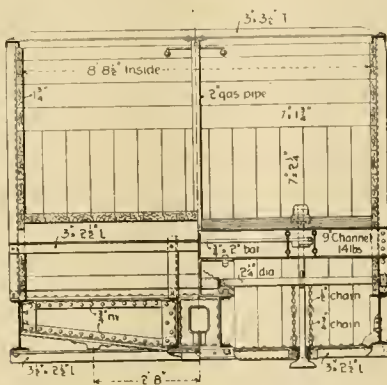
Cross-Sections of Coal and Ore Car.
