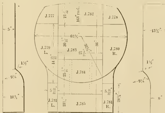
Fig. 16.—Back Tube Sheet, Male.
