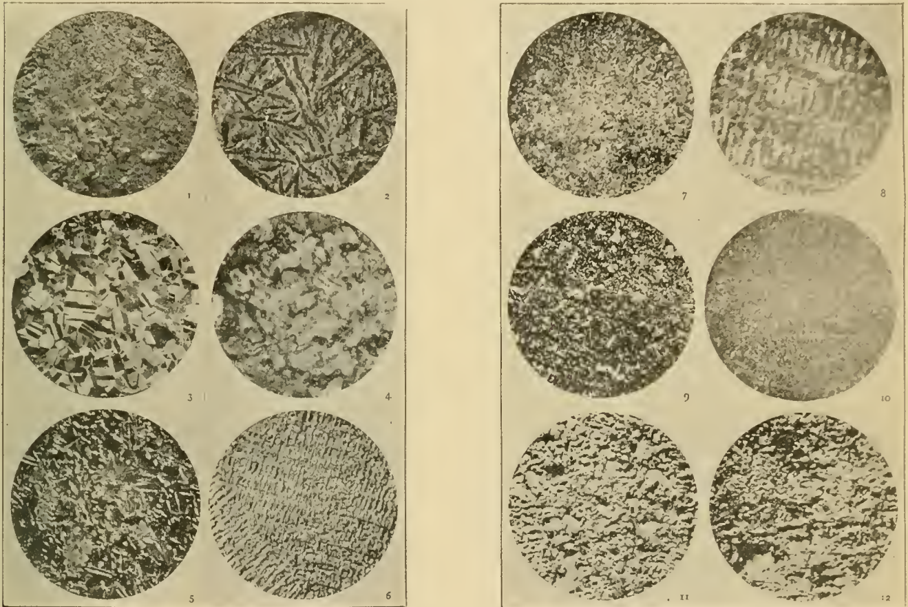
Figs. 1.—Antimonial lead. 2.—Tin and zinc with little copper and lead. 3.—Copper and zinc. 4.—Copper, zinc, tin, lead, iron. 5.—Copper and zinc with little lead (manganese used as deoxidizer). 6.—Copper and tin. 7.—Copper, tin, lead and phosphorus (1st melting). 8.—Copper, tin, lead and phosphorus (after repeated meltings). 9.—Copper, tin and lead (1st melting). 10.—Copper, tin and lead (after repeated meltings). 11.—Copper, tin and lead, showing liquation of lead. 12.—Copper, tin and lead, showing liquation of lead.
