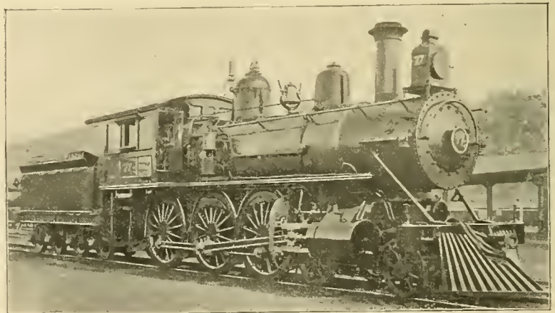
Locomotive with Piston Valves.—N. & W. Rv.
