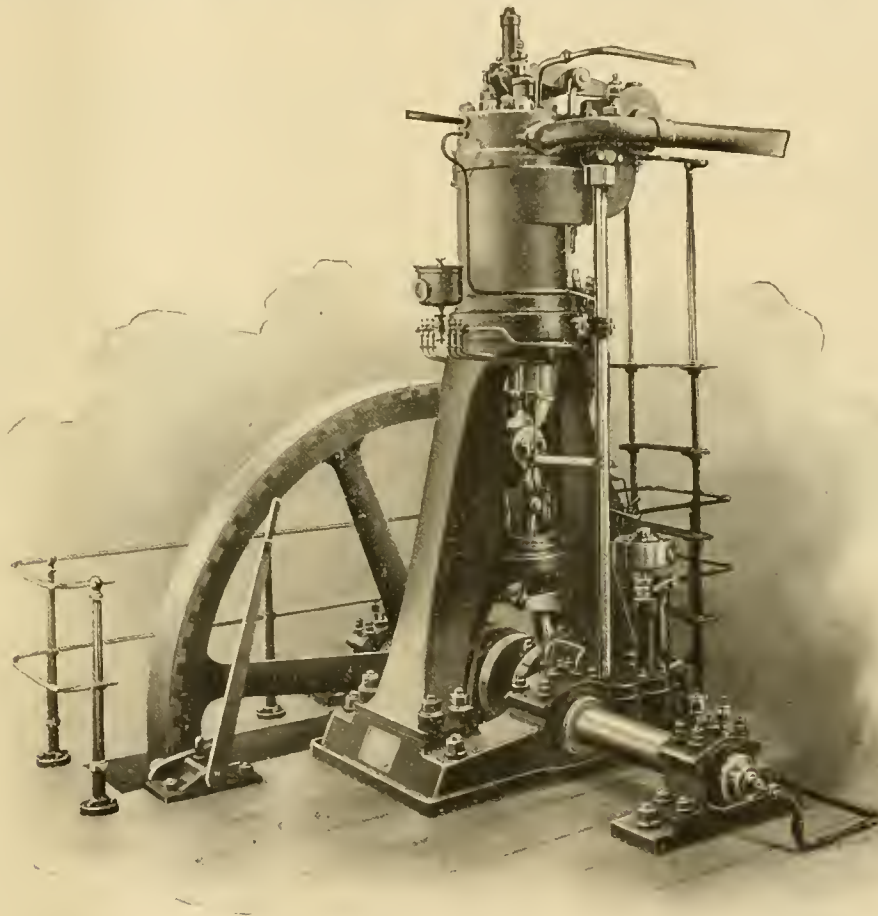
Fig. 1.—A 120-Horse-Power Diesel Motor.
