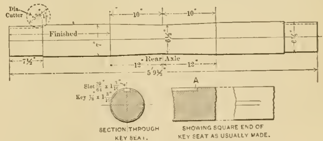
Improved Method of Cutting Key Ways.
