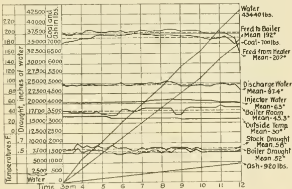
Fig. 1—Boiler Test.
