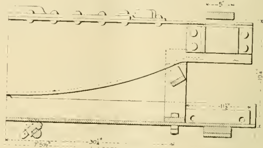
Truck Bolster.
