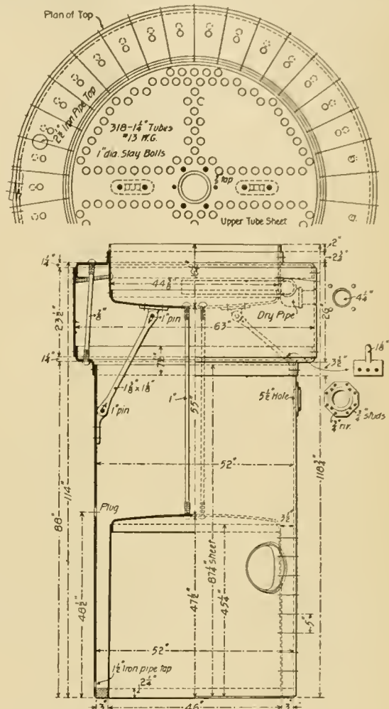
Motor Car Boiler, Schenectady Locomotive Works.
