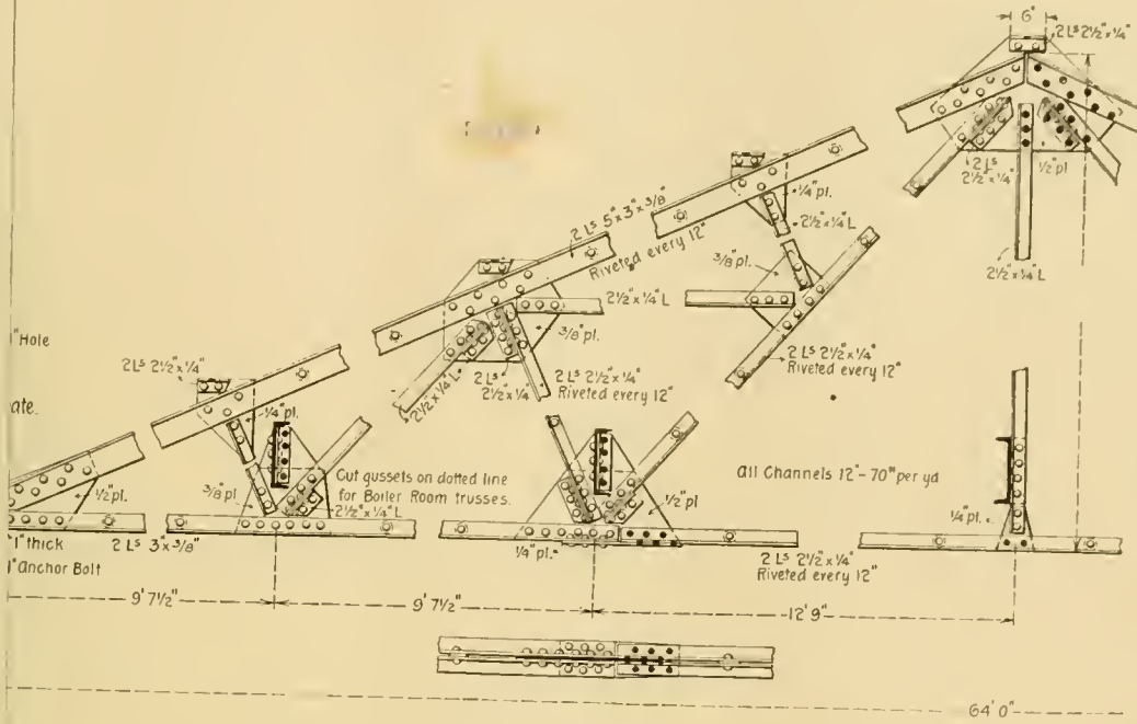
Roof Truss of Power House.
