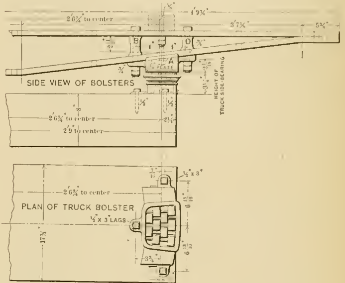
Side Bearing Fitted to Lake Shore Baggage Cars.
