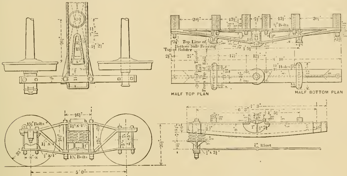
New Standard Truck and Body Bolsters—Seaboard Air Line. BY THE AMERICAN STEEL FOUNDRY CO.
