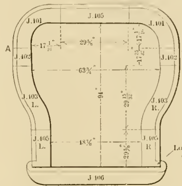
Fig. 13.—Female Die, Back Head.
