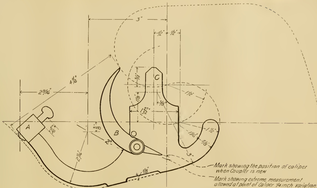
A New Coupler Gauge to Show Allowable Wear.
