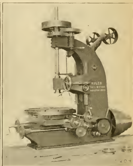
Fig. 2.—Vertical Milling Machine.
