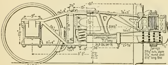
Metal Truck.
