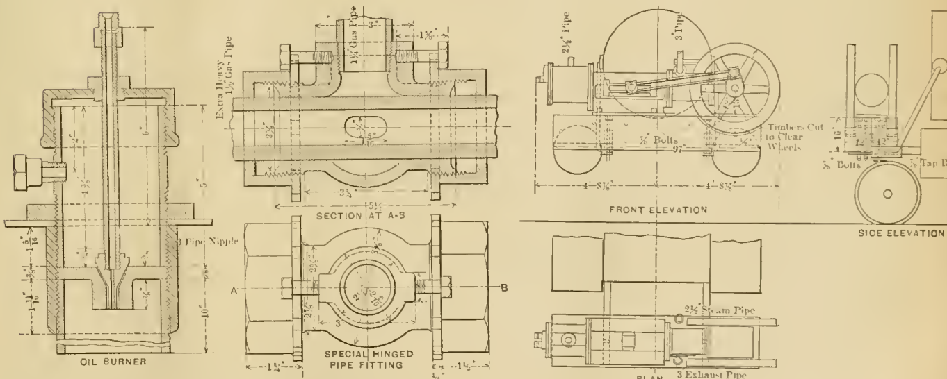
Details of Oil Burner and Hinge Joint.
