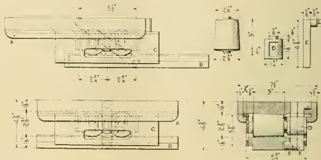
The New Susemihl-Torrey, Low Roller Side Bearing.
