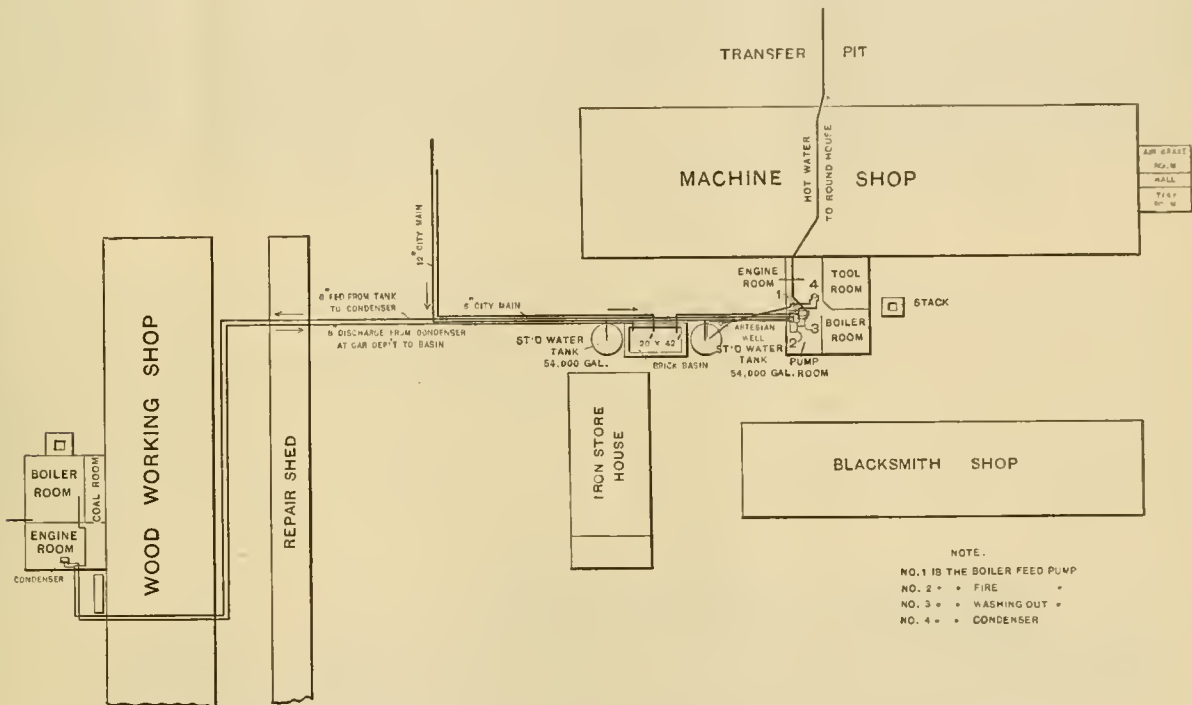
Condensers for Shop Engines—Chicago, Milwaukee & St. Paul Railway.
