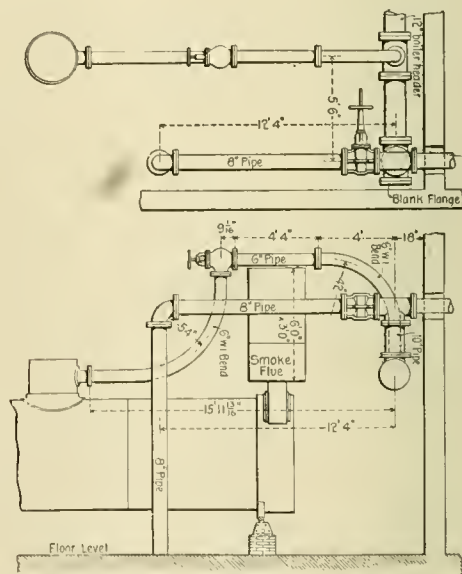
Connections from Boilers to Header.
