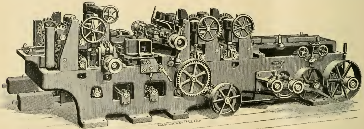
A New Six Roll Flooring Machine.
