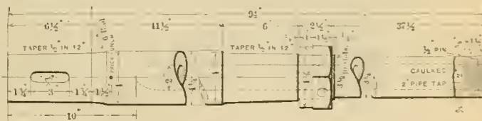
Hollow Piston Rod.
