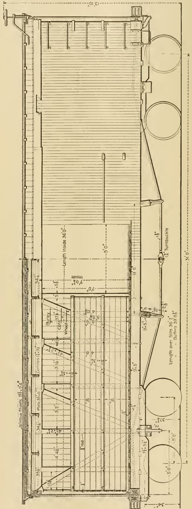
Box Car, 70,000 Lbs. Capacity—Northern Pacific Railway.
