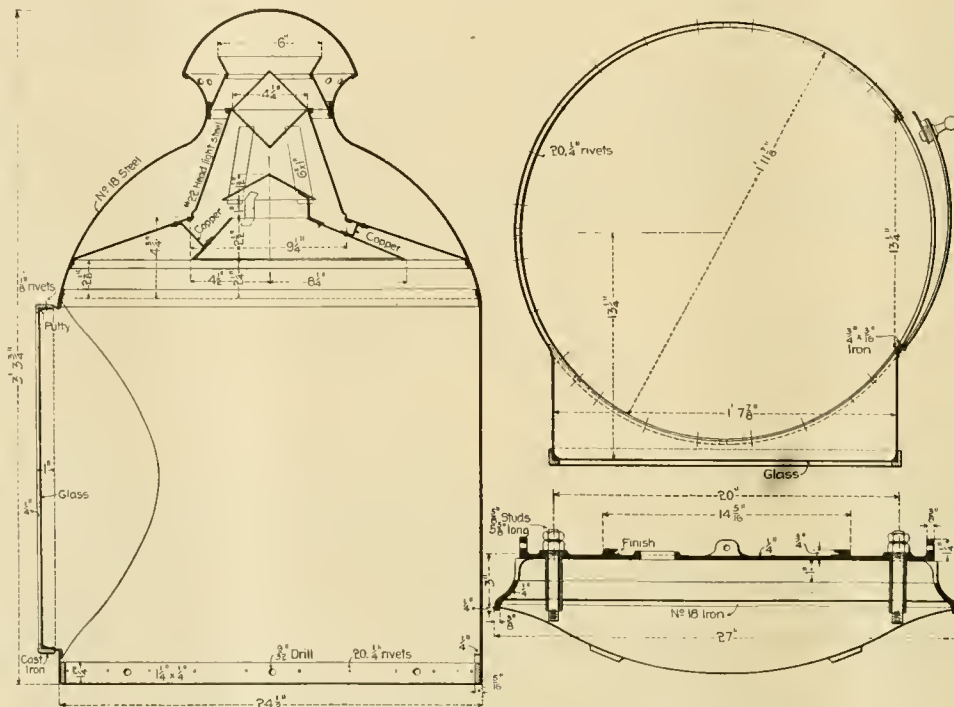
Circular Steel Headlight.—Chicago, Milwaukee & St. Paul Ry.
