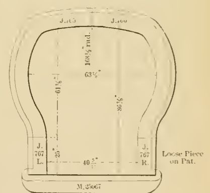
Fig. 17.—Female Die.
