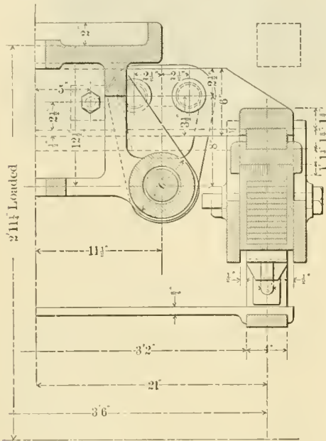
Engine Truck Suspension.
