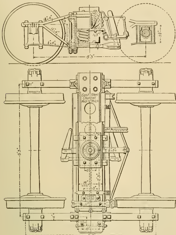
Truck Fitted with Wooden Bolster.
