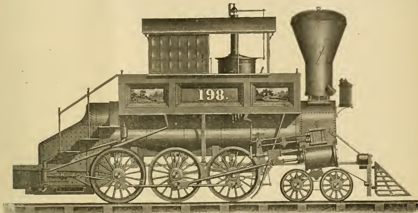
Hayes' Ten-Wheel Locomotive.
