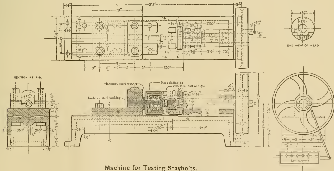
Machine for Testing Staybolts.
