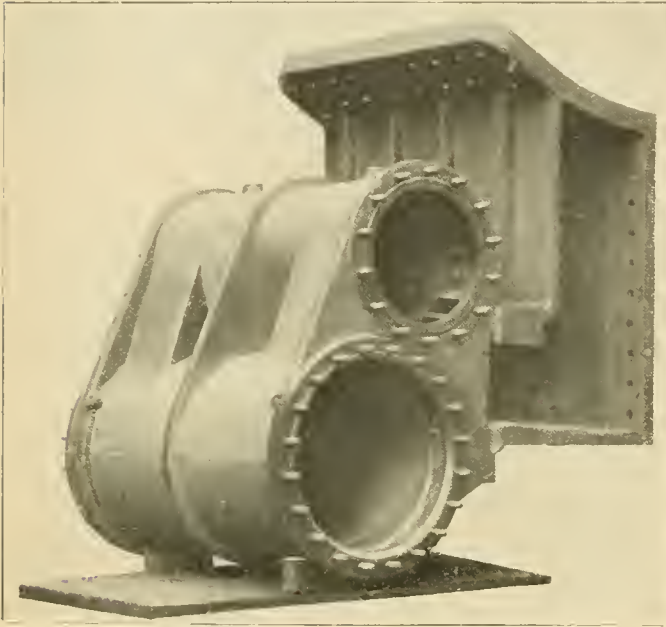
Cylinder of Great Northern Locomotive.
