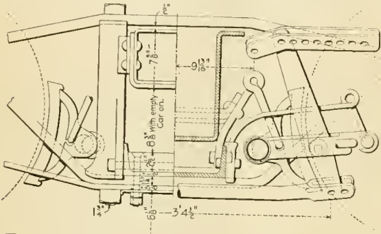
Partial End View of Truck.
