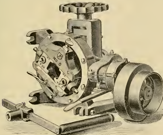
Armstrong Pipe Machine with Power Attachment.
