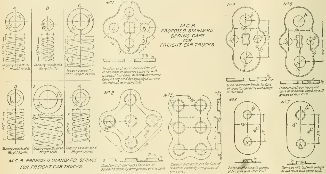
Proposed Standard Freight Truck Springs.
