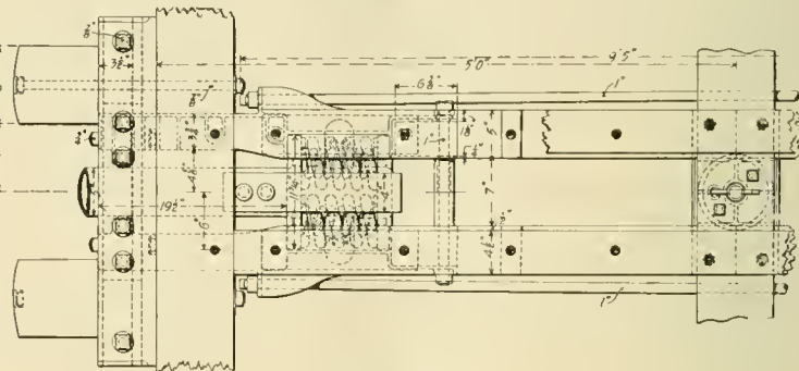
Draft Rigging.
