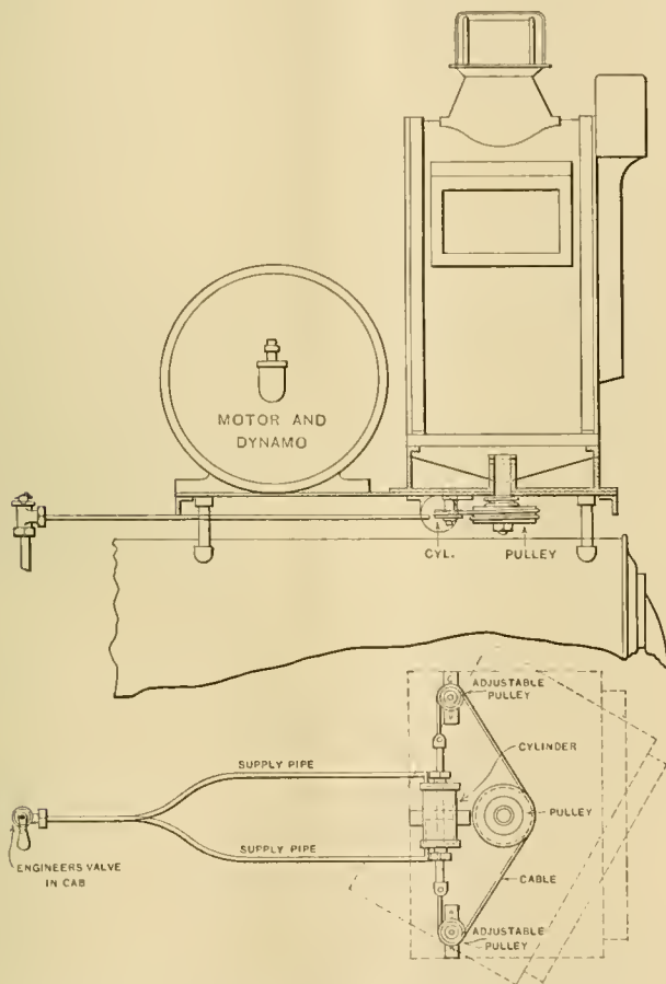
Search-light Attachment for Locomotive Headlights.
