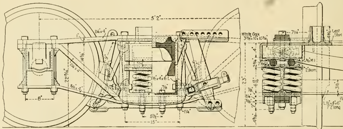
Sections and Partial Elevation of Truck.
