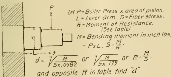
Diagram and Formulae for Crank Pins.
