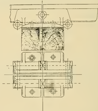
Webb's Rail Joint.
