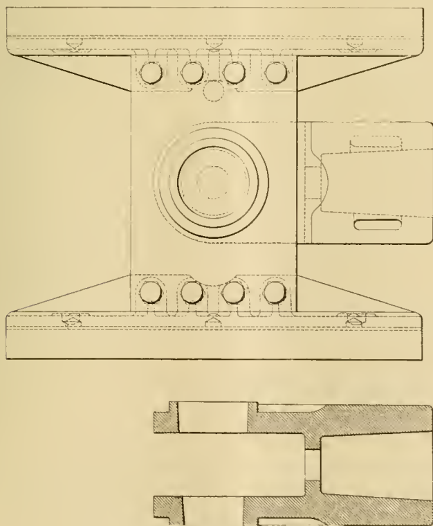
Articulated Crosshead—N. & W. Ry.
