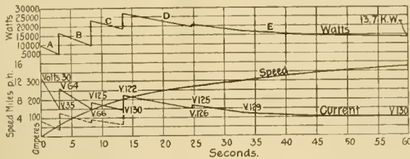
Fig. 4—Average of Five Acceleration Tests.
