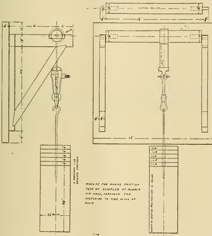
Apparatus for Testing "Friction" of Hose.
