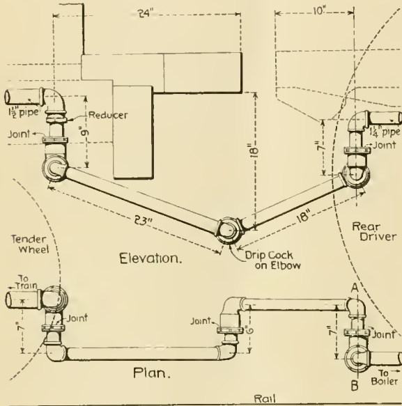
Plan and Elevation of Steam Heat Conduit.
