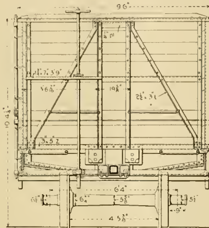
End Elevations and Sections—Coal and Ore Car.
