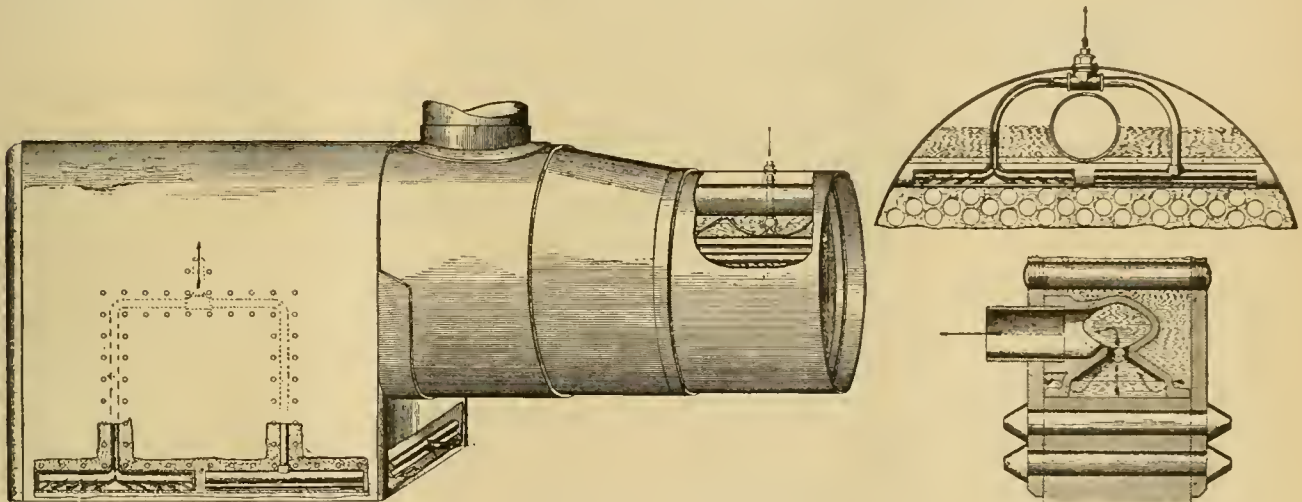
The Hornish Mechanical Locomotive Boiler Cleaner.
