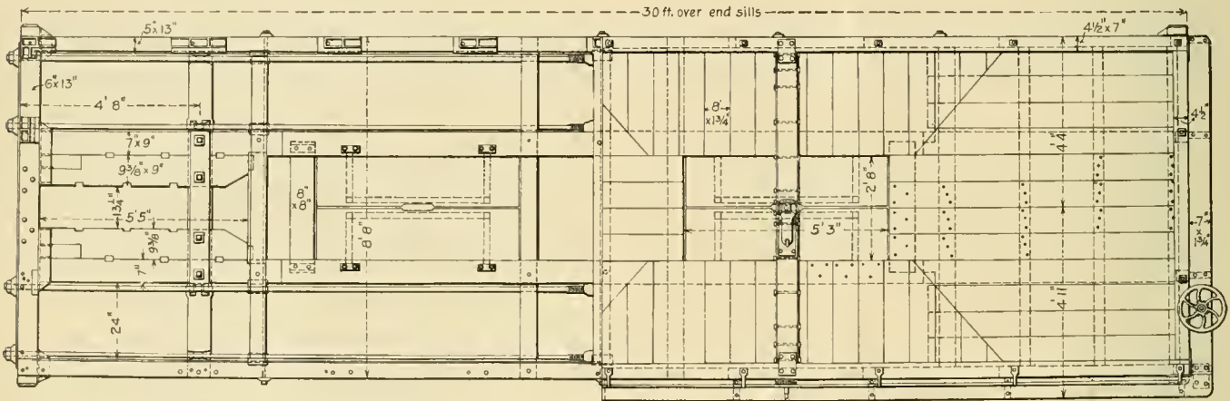
Half Plan of Bottom Framing.
