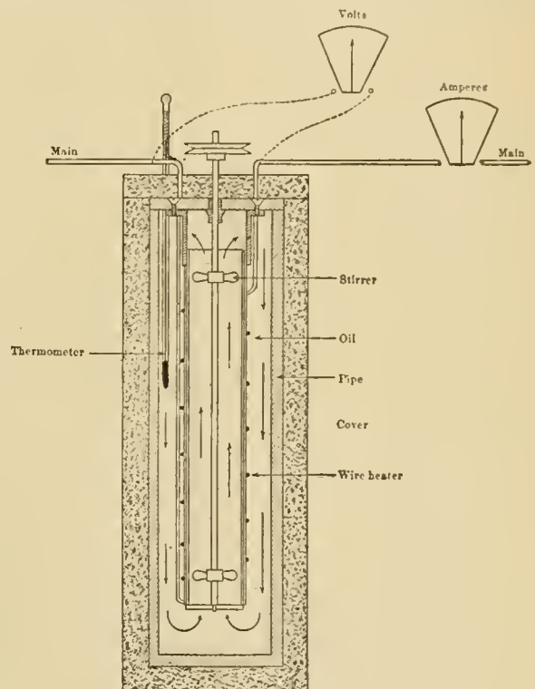
Apparatus Used by Prof. Norton.
