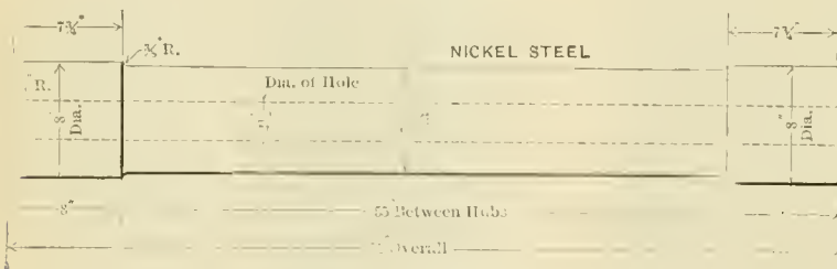
Hollow Driving Axle.
