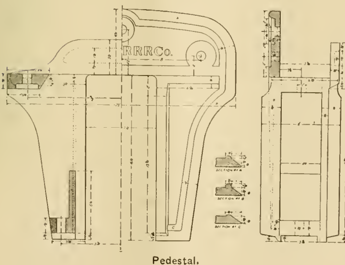
Pedestal.
