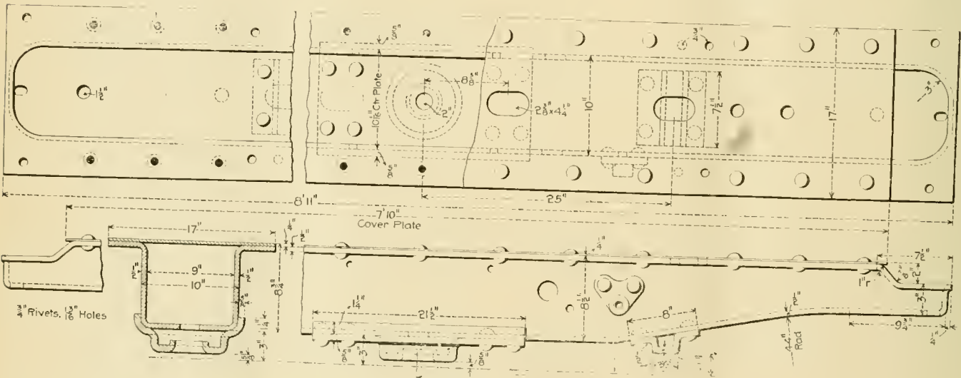
Body Bolster.
