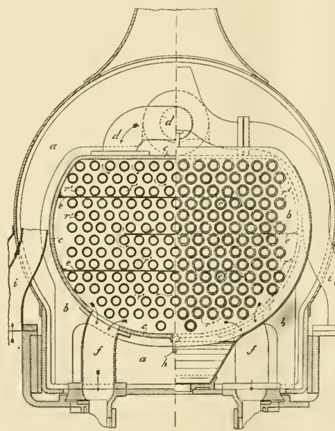
A Superheater for Locomotives.
