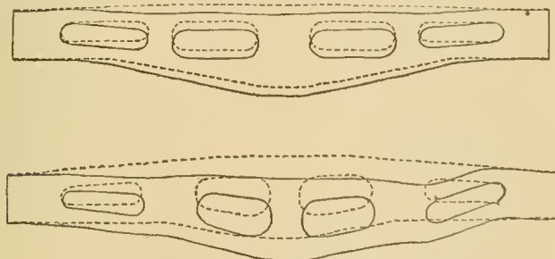
FIG. 3.—Distortion of the Bolsters in Tests.
