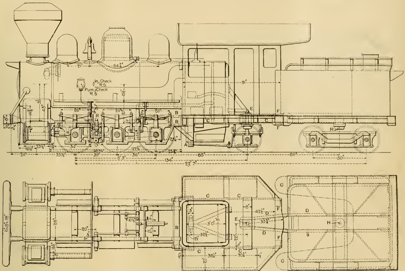
Narrow Gauge Locomotive, Cauca Railway, United States of Colombia. Built by the BALDWIN LOCOMOTIVE WORKS, from Designs by M. N. FORNEY, M. E.
