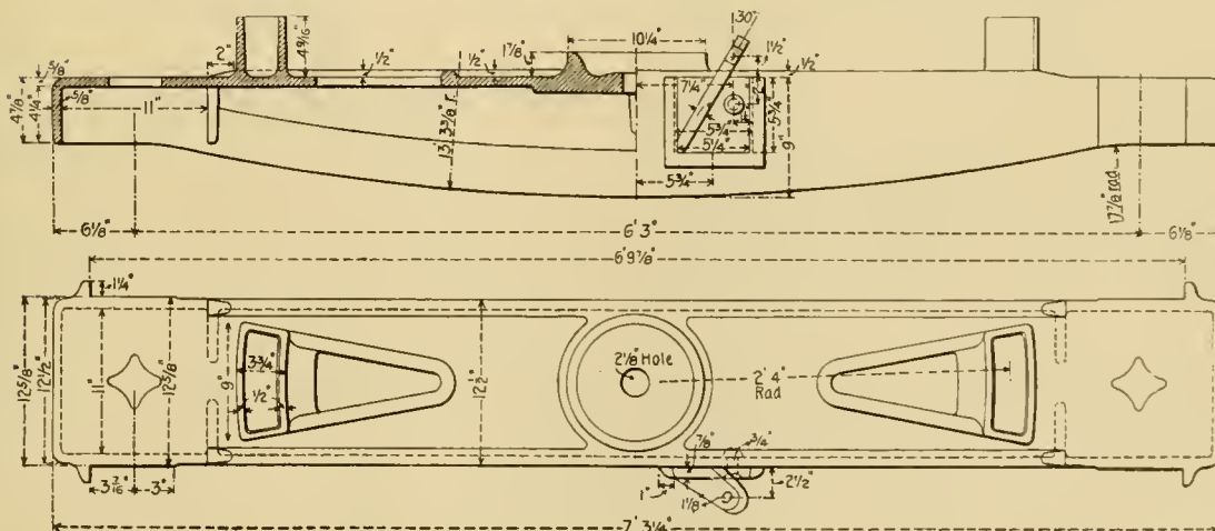
Cast Steel Truck Bolster.
