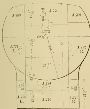
Fig. 15.—Back Tube Sheet Holder Plate.
