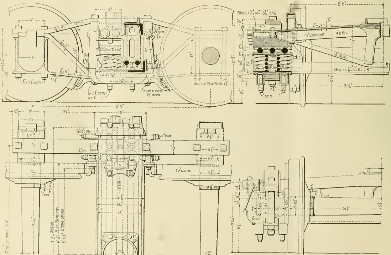
Details of Truck and Truck Bolster.
