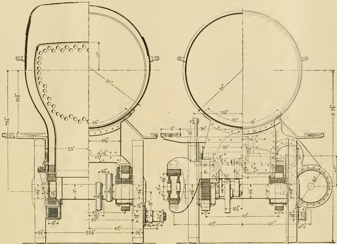
Transverse Sections.
