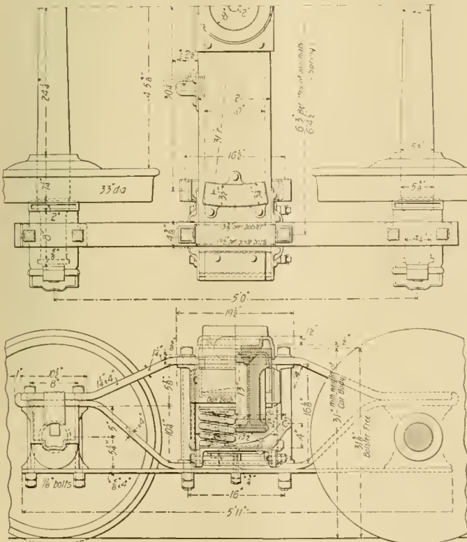
Trucks.
