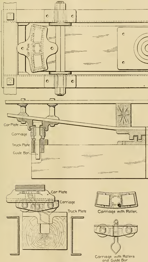
The Susemihl-Torrey Side Bearing.
