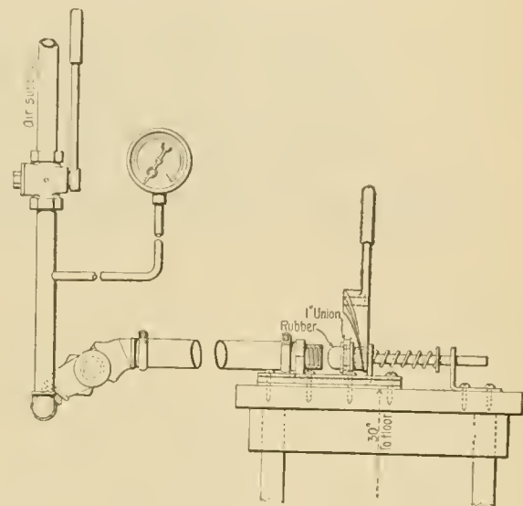
Air Hose Testing Apparatus.
