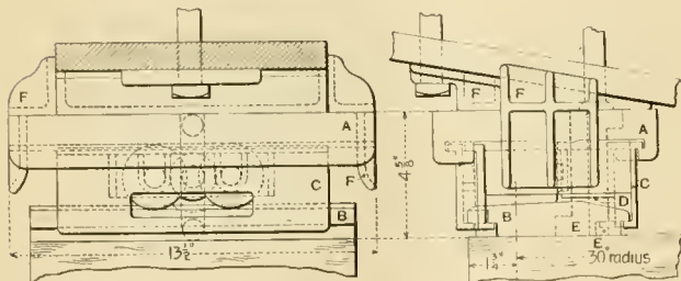
The New Susemihl-Torrey, Low Roller Side Bearing.
