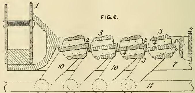
Locomotive Grates—M. N. Forney.
