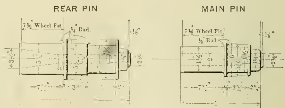
Hollow Crank Pins.
