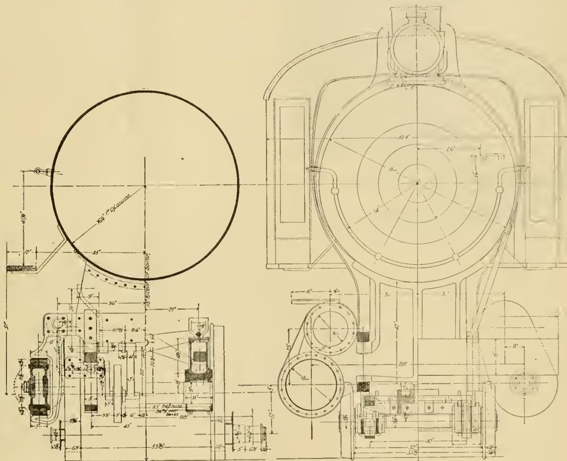
Front Elevation and Sections through Running Gear. Powerful Simple Locomotives—Great Northern Railway.
