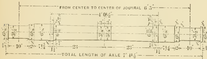
Axle for 100,000 Lbs. Capacity Cars.
