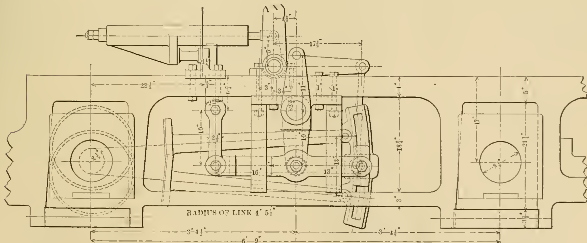
Valve Motion—Showing Connection Between Links and Rockers.
