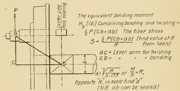
Diagram and Formulae for Driving Axles.
