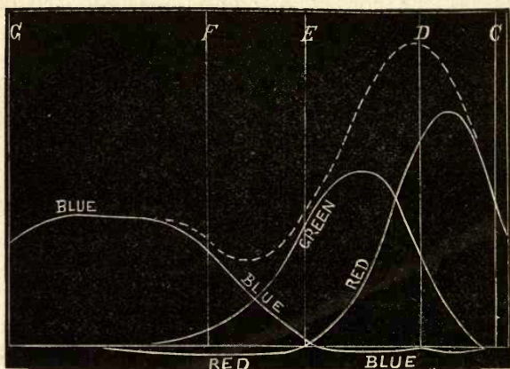
FIG. 37.—Maxwell's Curves of Colour Sensations.
