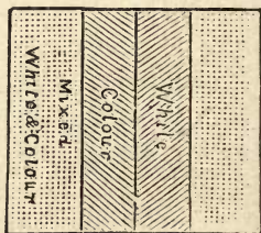
FIG. 45.—Method of showing Contrast Colours.
