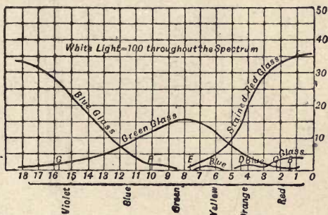
FIG. 17.—Absorption by Red, Blue, and Green Glasses.
