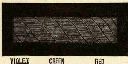
FIG. 9.—Interference Bands.
