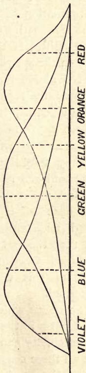
FIG. 34.—Curves of Colour Sensations.
