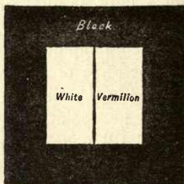
FIG. 12.—Rectangles of White and Vermilion.
