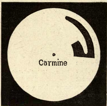
FIG. 24.—Template of Carmine.
