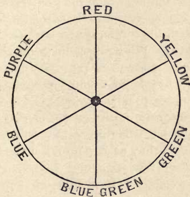
FIG. 38.—Chromatic Circle.
