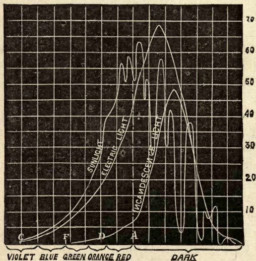
FIG. 5.—Heating effect of different Sources of Radiation.
