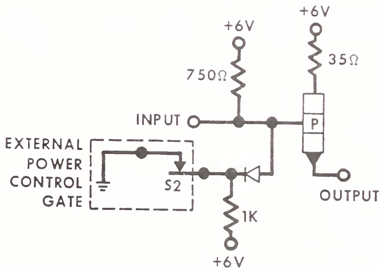
FIGURE 5. Line Drivers
