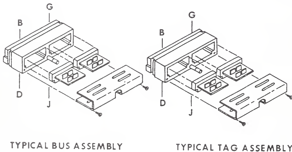
FIGURE 19. Terminator Assemblies
